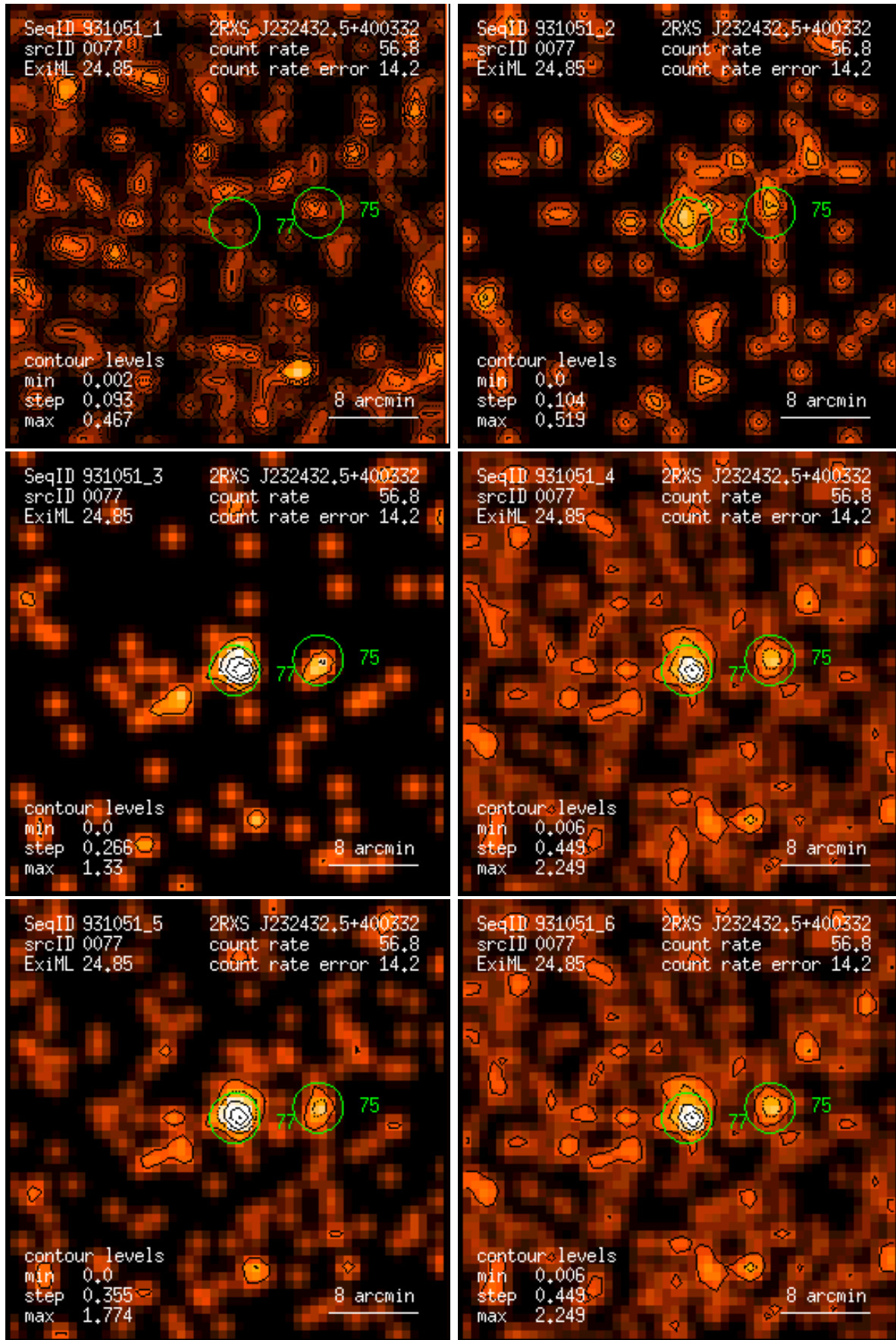
Figure 77: RASS 931051: detection 0077: band rate images, Gaussian filter: (1) PSPC channels 11 – 41, (2) 52 – 90, (3) 91 – 201, (4) 11 – 235, (5) 52 – 201, (6) 11 – 201. Broad band rates in counts/ks. Band rate contour levels in counts/ks/arcmin 2 .
