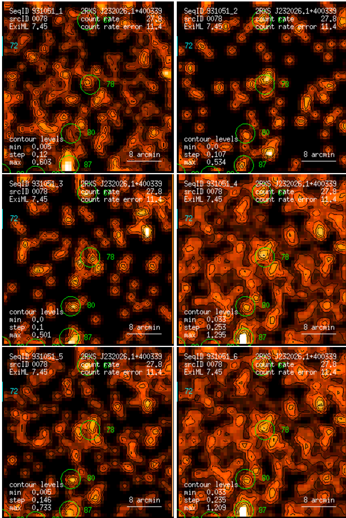
Figure 78: RASS 931051: detection 0078: band rate images, Gaussian filter: (1) PSPC channels 11 – 41, (2) 52 – 90, (3) 91 – 201, (4) 11 – 235, (5) 52 – 201, (6) 11 – 201. Broad band rates in counts/ks. Band rate contour levels in counts/ks/arcmin 2 .
