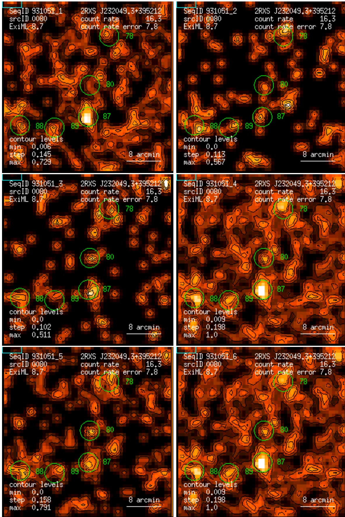
Figure 80: RASS 931051: detection 0080: band rate images, Gaussian filter: (1) PSPC channels 11 – 41, (2) 52 – 90, (3) 91 – 201, (4) 11 – 235, (5) 52 – 201, (6) 11 – 201. Broad band rates in counts/ks. Band rate contour levels in counts/ks/arcmin 2 .
