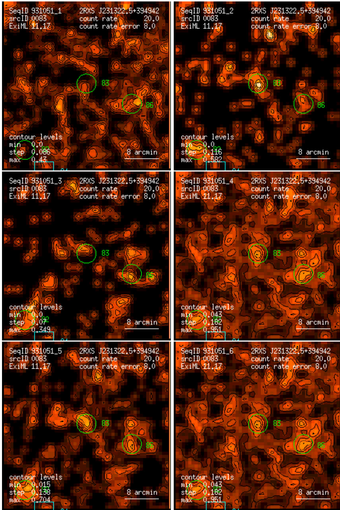
Figure 83: RASS 931051: detection 0083: band rate images, Gaussian filter: (1) PSPC channels 11 – 41, (2) 52 – 90, (3) 91 – 201, (4) 11 – 235, (5) 52 – 201, (6) 11 – 201. Broad band rates in counts/ks. Band rate contour levels in counts/ks/arcmin 2 .
