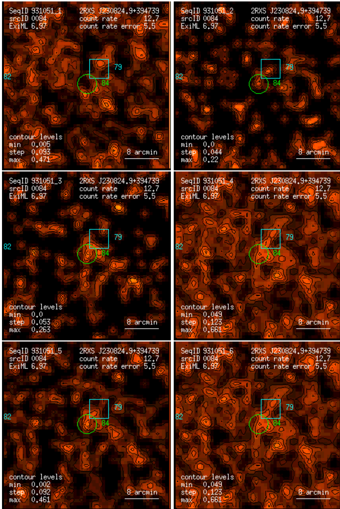
Figure 84: RASS 931051: detection 0084: band rate images, Gaussian filter: (1) PSPC channels 11 – 41, (2) 52 – 90, (3) 91 – 201, (4) 11 – 235, (5) 52 – 201, (6) 11 – 201. Broad band rates in counts/ks. Band rate contour levels in counts/ks/arcmin 2 .
