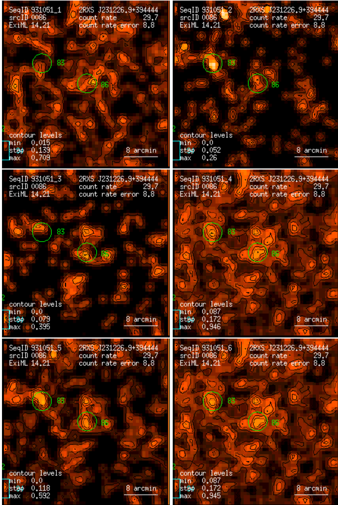
Figure 86: RASS 931051: detection 0086: band rate images, Gaussian filter: (1) PSPC channels 11 – 41, (2) 52 – 90, (3) 91 – 201, (4) 11 – 235, (5) 52 – 201, (6) 11 – 201. Broad band rates in counts/ks. Band rate contour levels in counts/ks/arcmin 2 .
