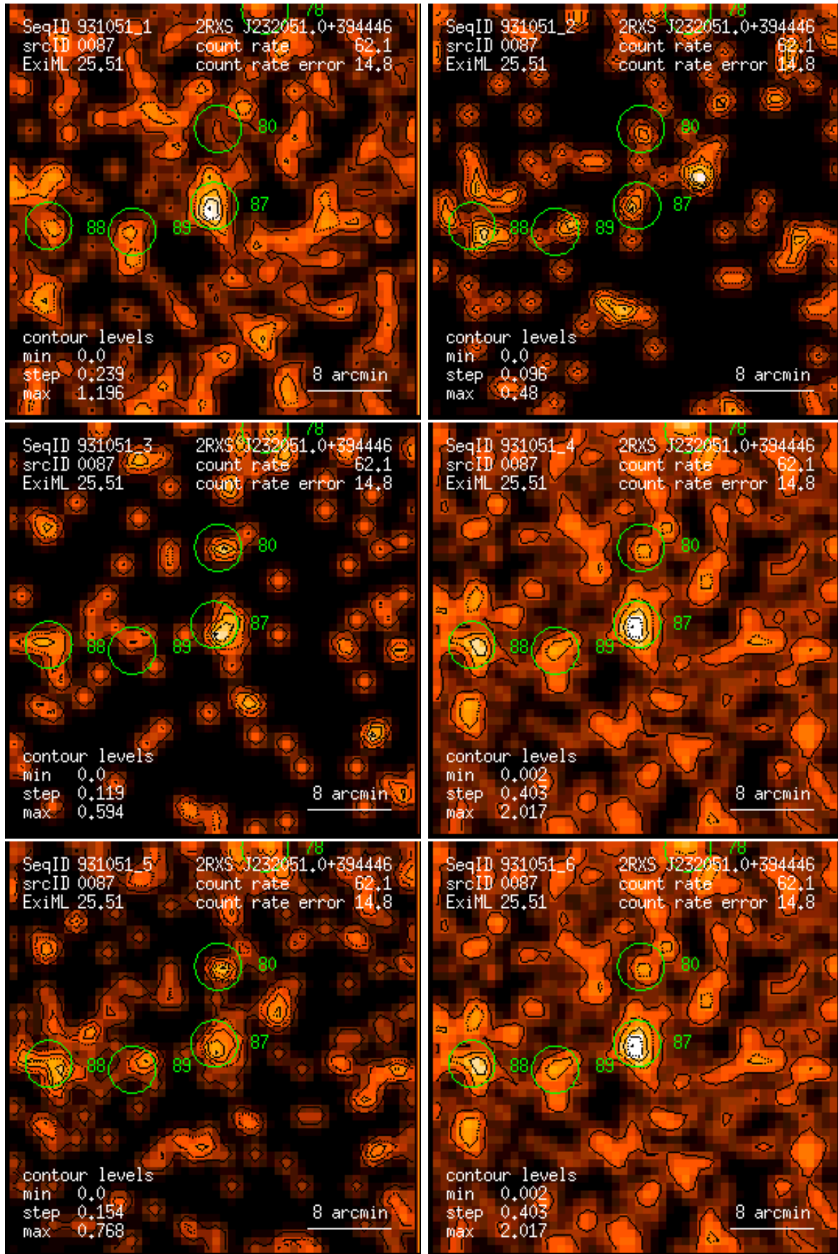
Figure 87: RASS 931051: detection 0087: band rate images, Gaussian filter: (1) PSPC channels 11 – 41, (2) 52 – 90, (3) 91 – 201, (4) 11 – 235, (5) 52 – 201, (6) 11 – 201. Broad band rates in counts/ks. Band rate contour levels in counts/ks/arcmin 2 .
