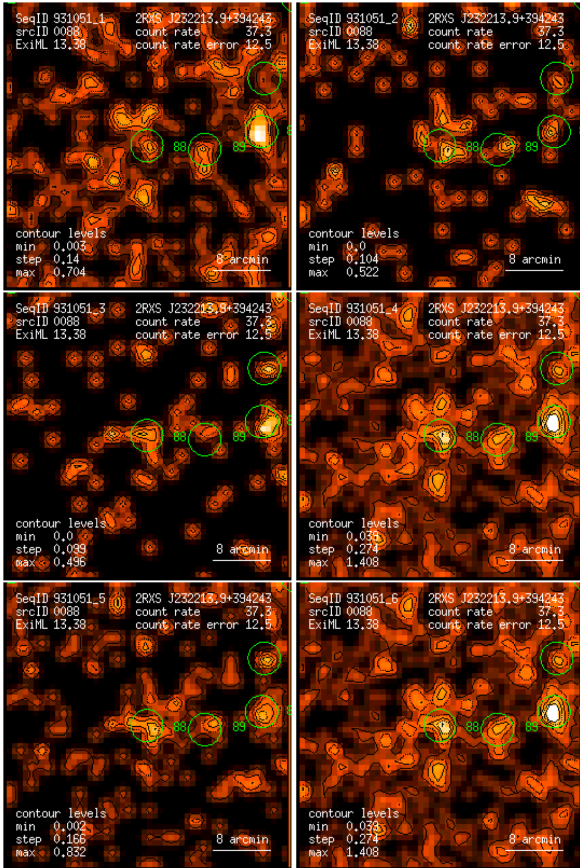
Figure 88: RASS 931051: detection 0088: band rate images, Gaussian filter: (1) PSPC channels 11 – 41, (2) 52 – 90, (3) 91 – 201, (4) 11 – 235, (5) 52 – 201, (6) 11 – 201. Broad band rates in counts/ks. Band rate contour levels in counts/ks/arcmin 2 .
