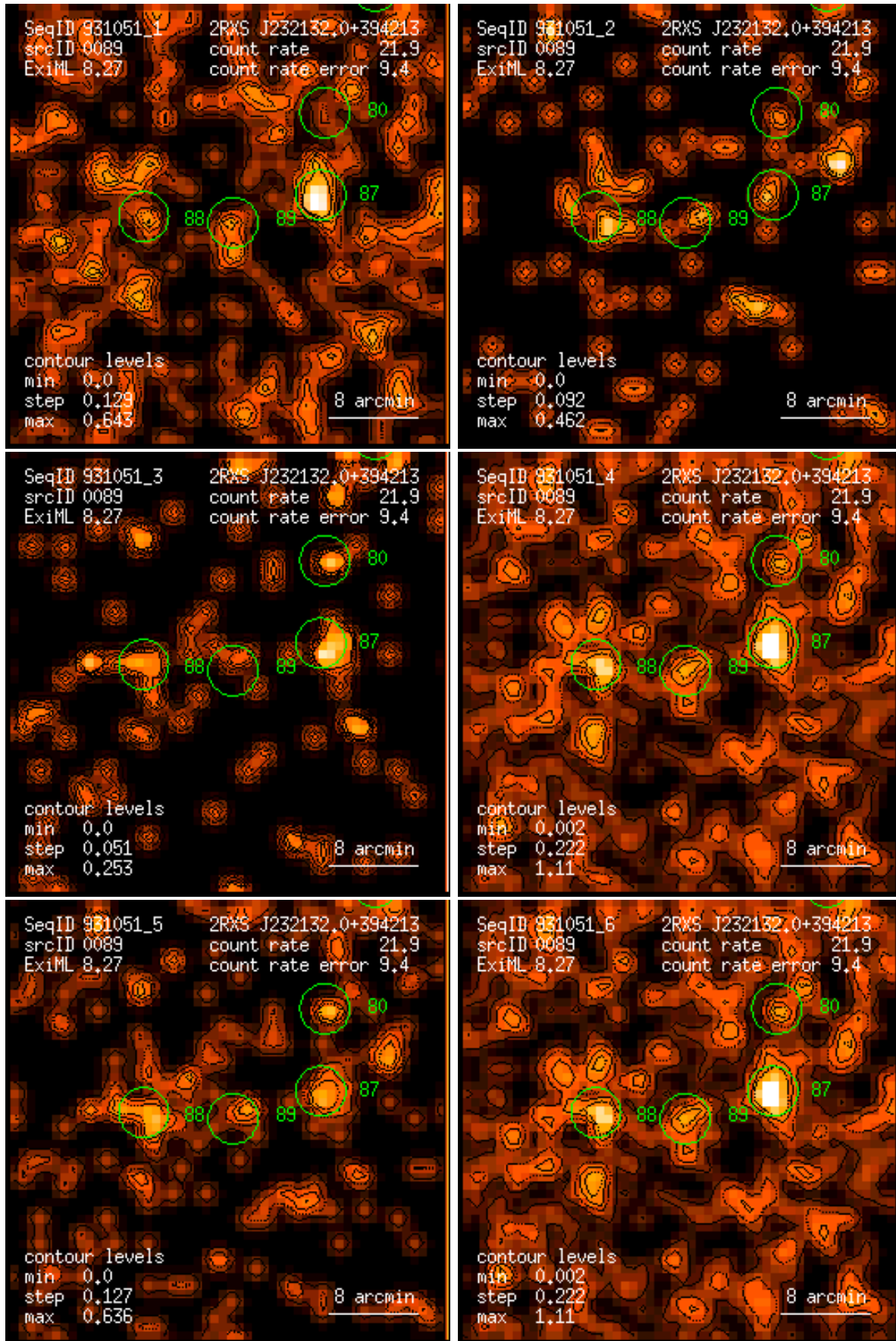
Figure 89: RASS 931051: detection 0089: band rate images, Gaussian filter: (1) PSPC channels 11 – 41, (2) 52 – 90, (3) 91 – 201, (4) 11 – 235, (5) 52 – 201, (6) 11 – 201. Broad band rates in counts/ks. Band rate contour levels in counts/ks/arcmin 2 .
