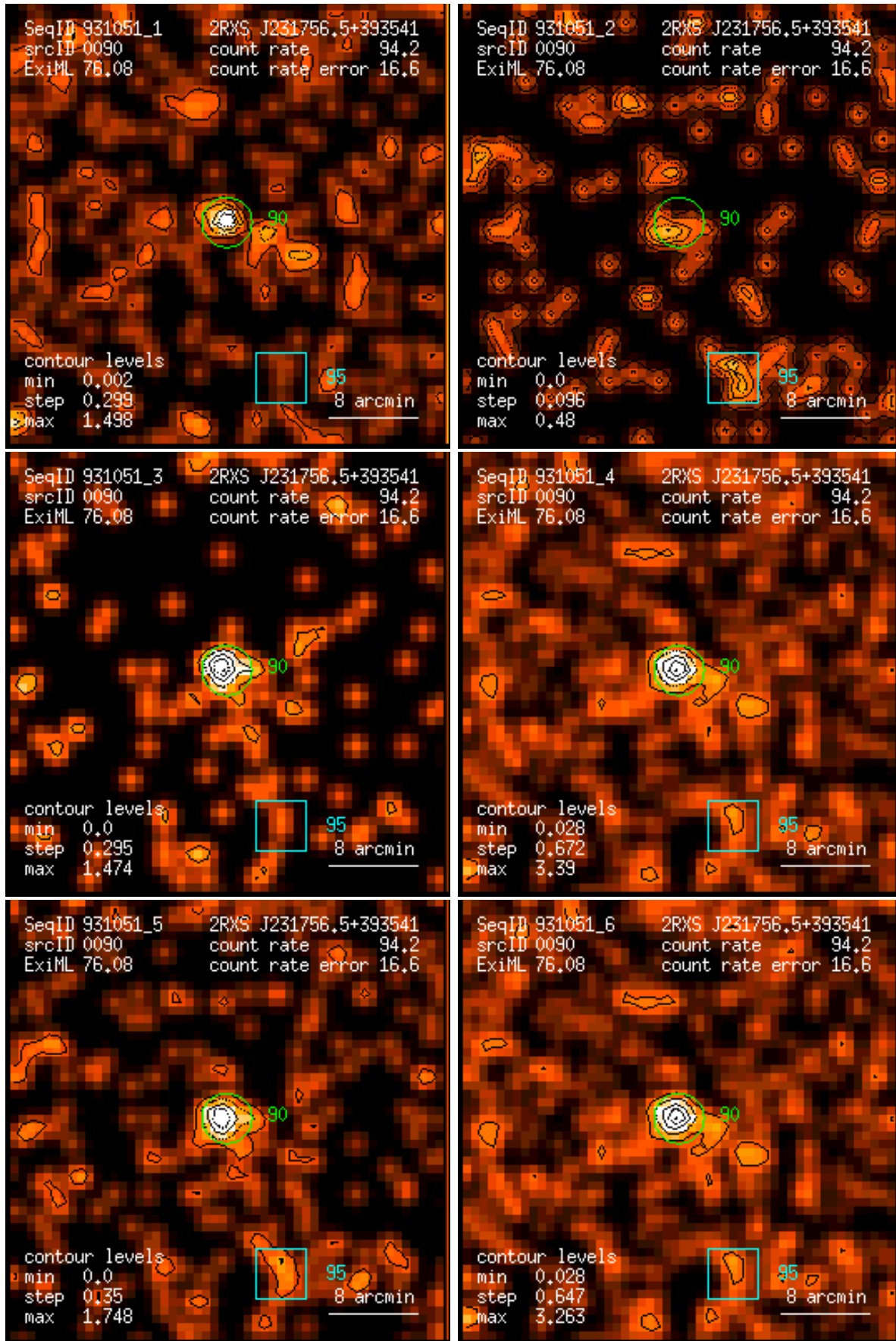
Figure 90: RASS 931051: detection 0090: band rate images, Gaussian filter: (1) PSPC channels 11 – 41, (2) 52 – 90, (3) 91 – 201, (4) 11 – 235, (5) 52 – 201, (6) 11 – 201. Broad band rates in counts/ks. Band rate contour levels in counts/ks/arcmin 2 .
