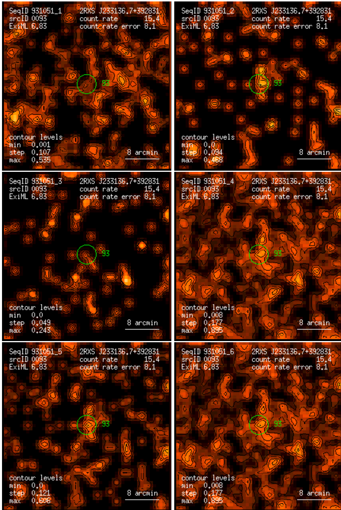
Figure 93: RASS 931051: detection 0093: band rate images, Gaussian filter: (1) PSPC channels 11 – 41, (2) 52 – 90, (3) 91 – 201, (4) 11 – 235, (5) 52 – 201, (6) 11 – 201. Broad band rates in counts/ks. Band rate contour levels in counts/ks/arcmin 2 .
