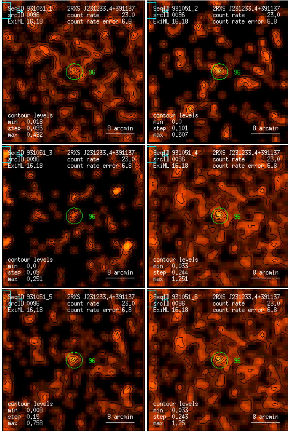
Figure 96: RASS 931051: detection 0096: band rate images, Gaussian filter: (1) PSPC channels 11 – 41, (2) 52 – 90, (3) 91 – 201, (4) 11 – 235, (5) 52 – 201, (6) 11 – 201. Broad band rates in counts/ks. Band rate contour levels in counts/ks/arcmin 2 .
