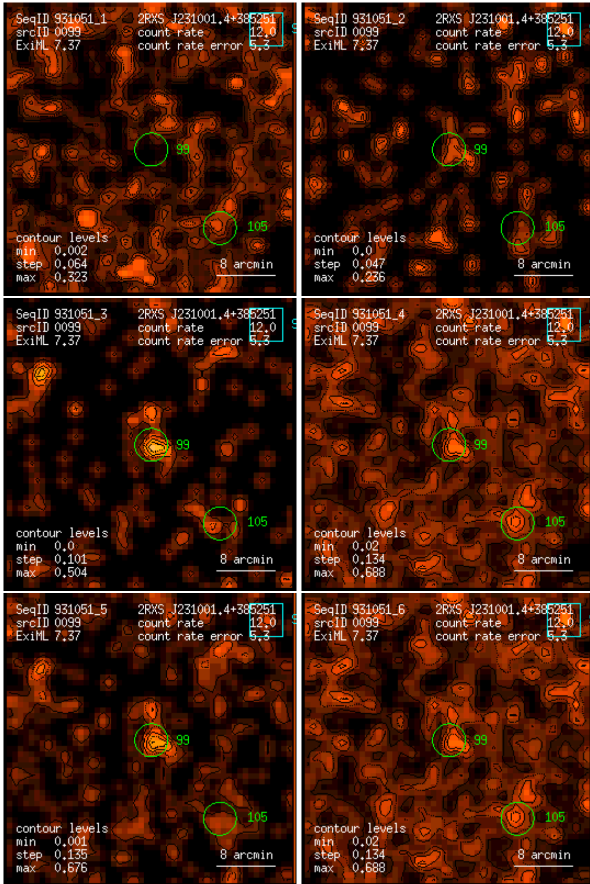
Figure 99: RASS 931051: detection 0099: band rate images, Gaussian filter: (1) PSPC channels 11 – 41, (2) 52 – 90, (3) 91 – 201, (4) 11 – 235, (5) 52 – 201, (6) 11 – 201. Broad band rates in counts/ks. Band rate contour levels in counts/ks/arcmin 2 .
