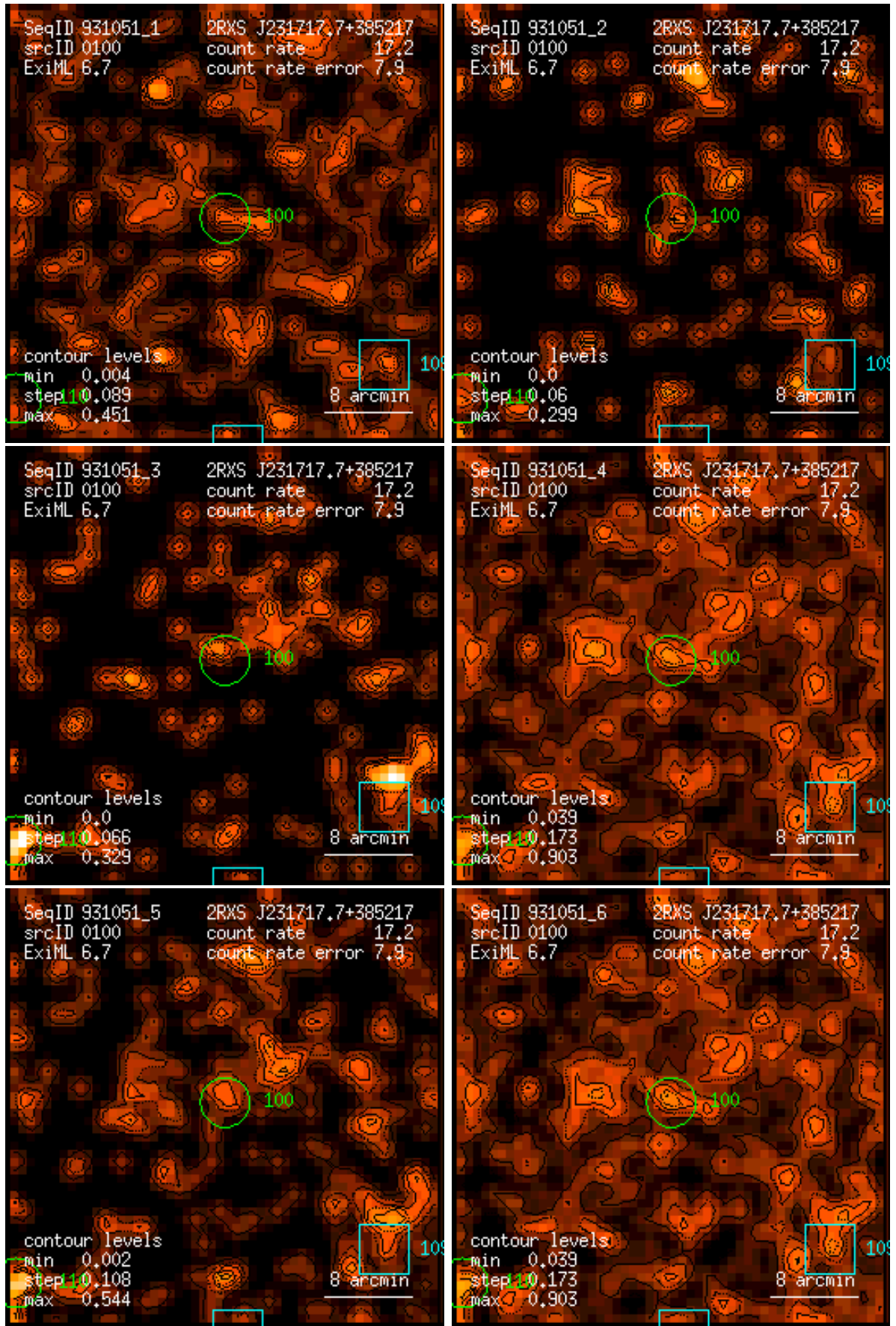
Figure 100: RASS 931051: detection 0100: band rate images, Gaussian filter: (1) PSPC channels 11 – 41, (2) 52 – 90, (3) 91 – 201, (4) 11 – 235, (5) 52 – 201, (6) 11 – 201. Broad band rates in counts/ks. Band rate contour levels in counts/ks/arcmin 2 .
