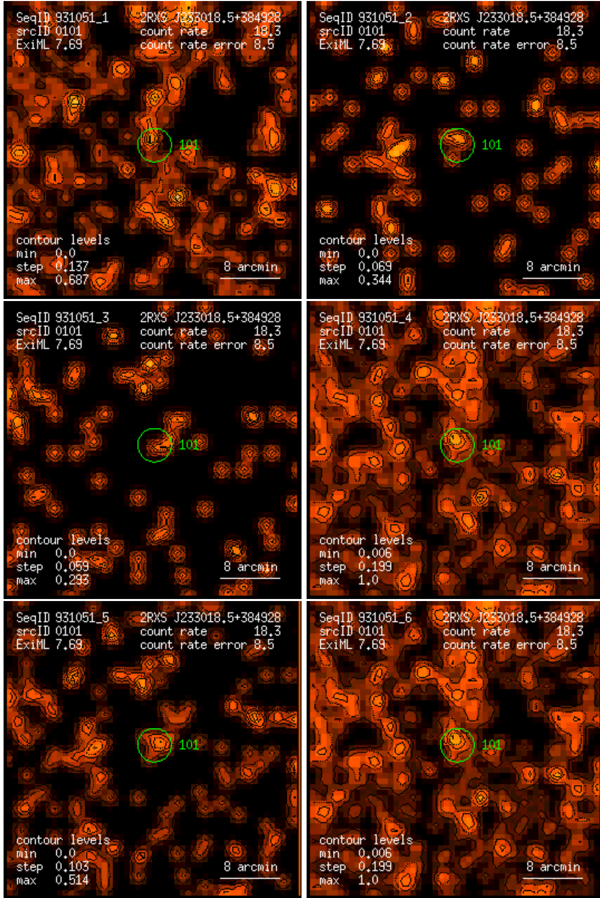
Figure 101: RASS 931051: detection 0101: band rate images, Gaussian filter: (1) PSPC channels 11 – 41, (2) 52 – 90, (3) 91 – 201, (4) 11 – 235, (5) 52 – 201, (6) 11 – 201. Broad band rates in counts/ks. Band rate contour levels in counts/ks/arcmin 2 .
