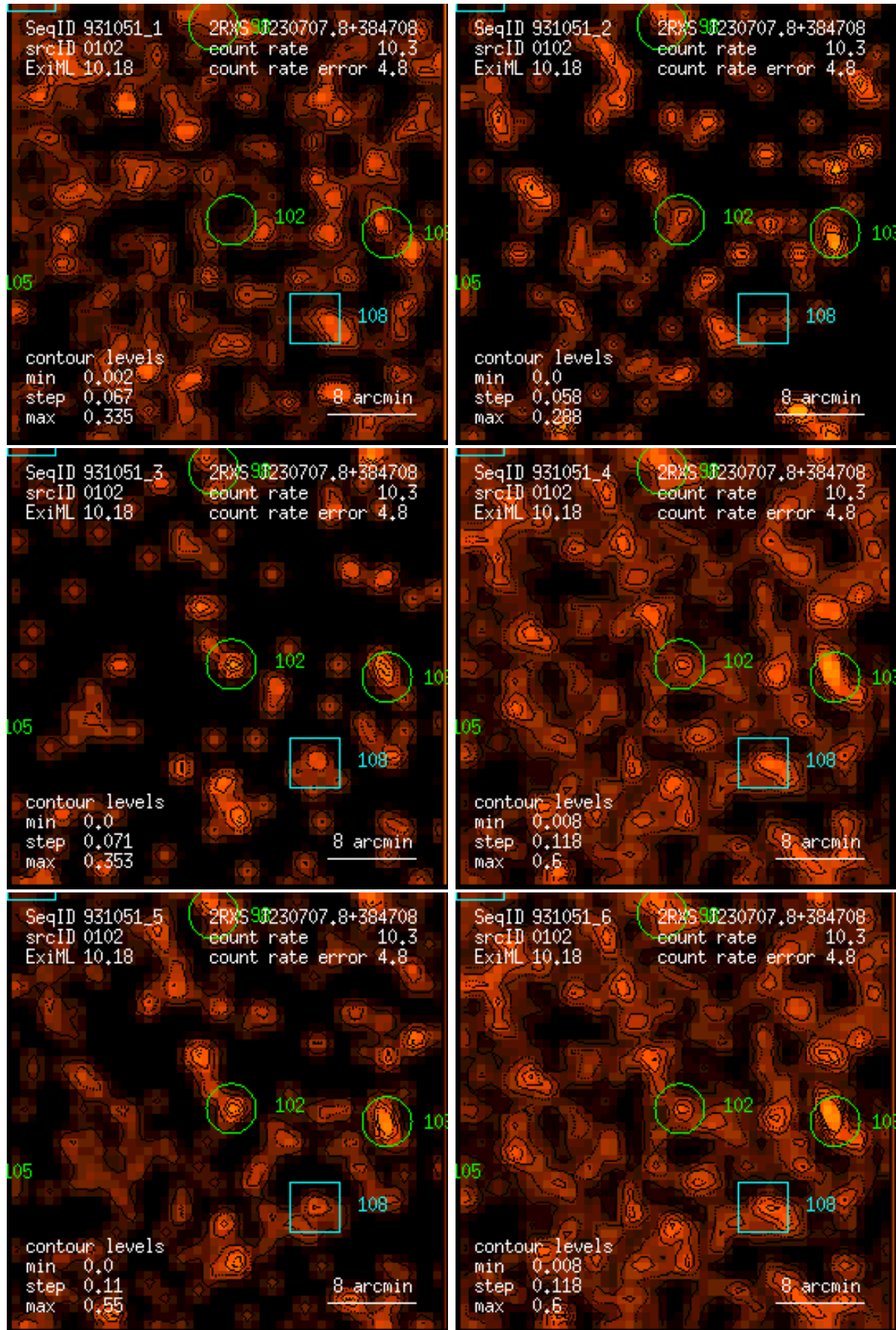
Figure 102: RASS 931051: detection 0102: band rate images, Gaussian filter: (1) PSPC channels 11 – 41, (2) 52 – 90, (3) 91 – 201, (4) 11 – 235, (5) 52 – 201, (6) 11 – 201. Broad band rates in counts/ks. Band rate contour levels in counts/ks/arcmin 2 .
