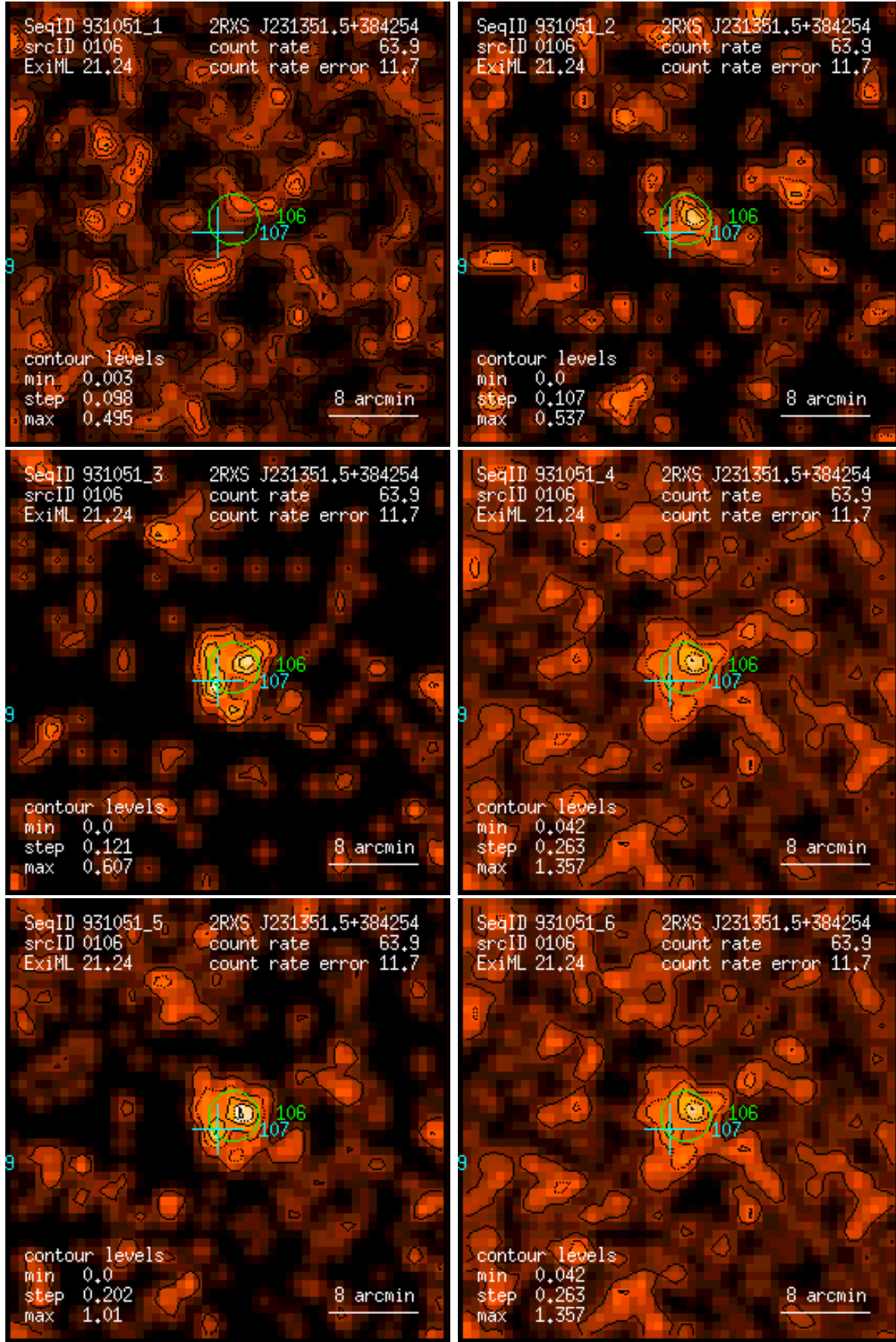
Figure 106: RASS 931051: detection 0106: band rate images, Gaussian filter: (1) PSPC channels 11 – 41, (2) 52 – 90, (3) 91 – 201, (4) 11 – 235, (5) 52 – 201, (6) 11 – 201. Broad band rates in counts/ks. Band rate contour levels in counts/ks/arcmin 2 .
