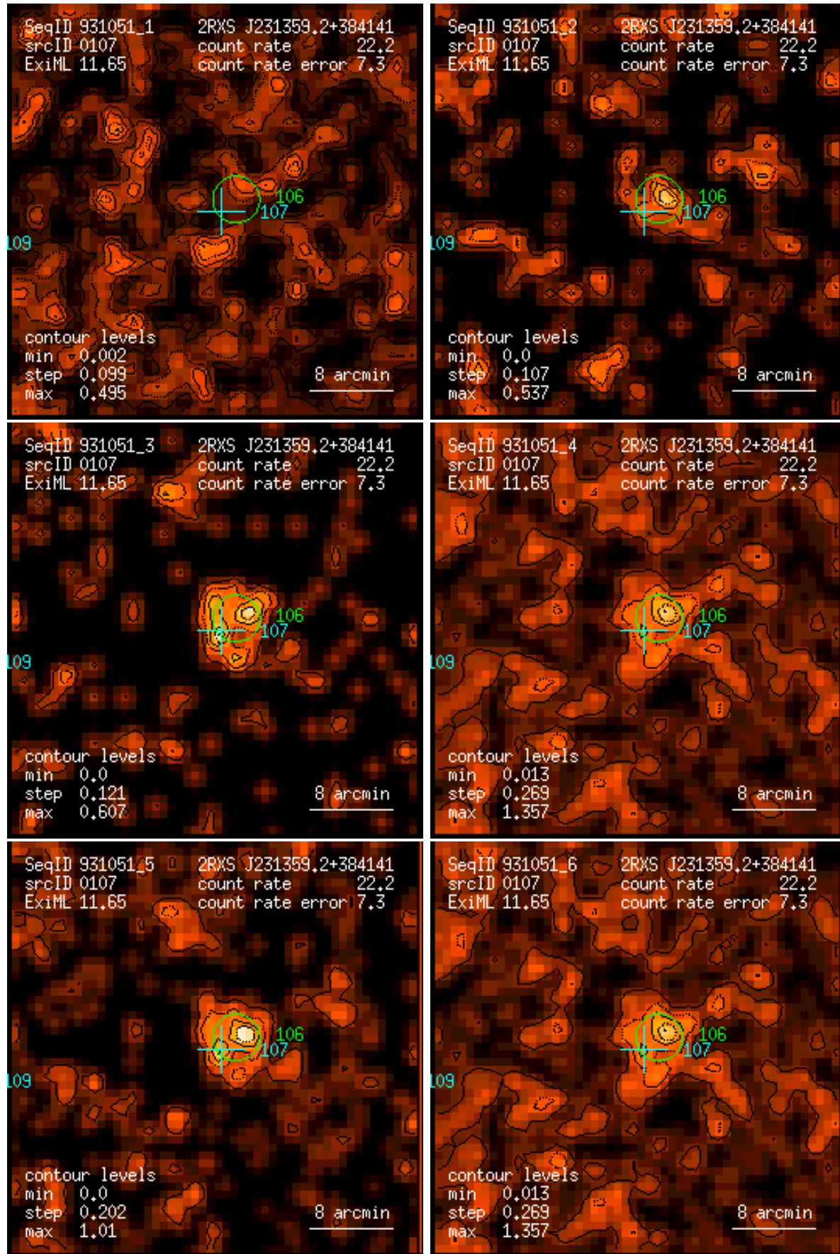
Figure 107: RASS 931051: detection 0107: band rate images, Gaussian filter: (1) PSPC channels 11 – 41, (2) 52 – 90, (3) 91 – 201, (4) 11 – 235, (5) 52 – 201, (6) 11 – 201. Broad band rates in counts/ks. Band rate contour levels in counts/ks/arcmin 2 .
