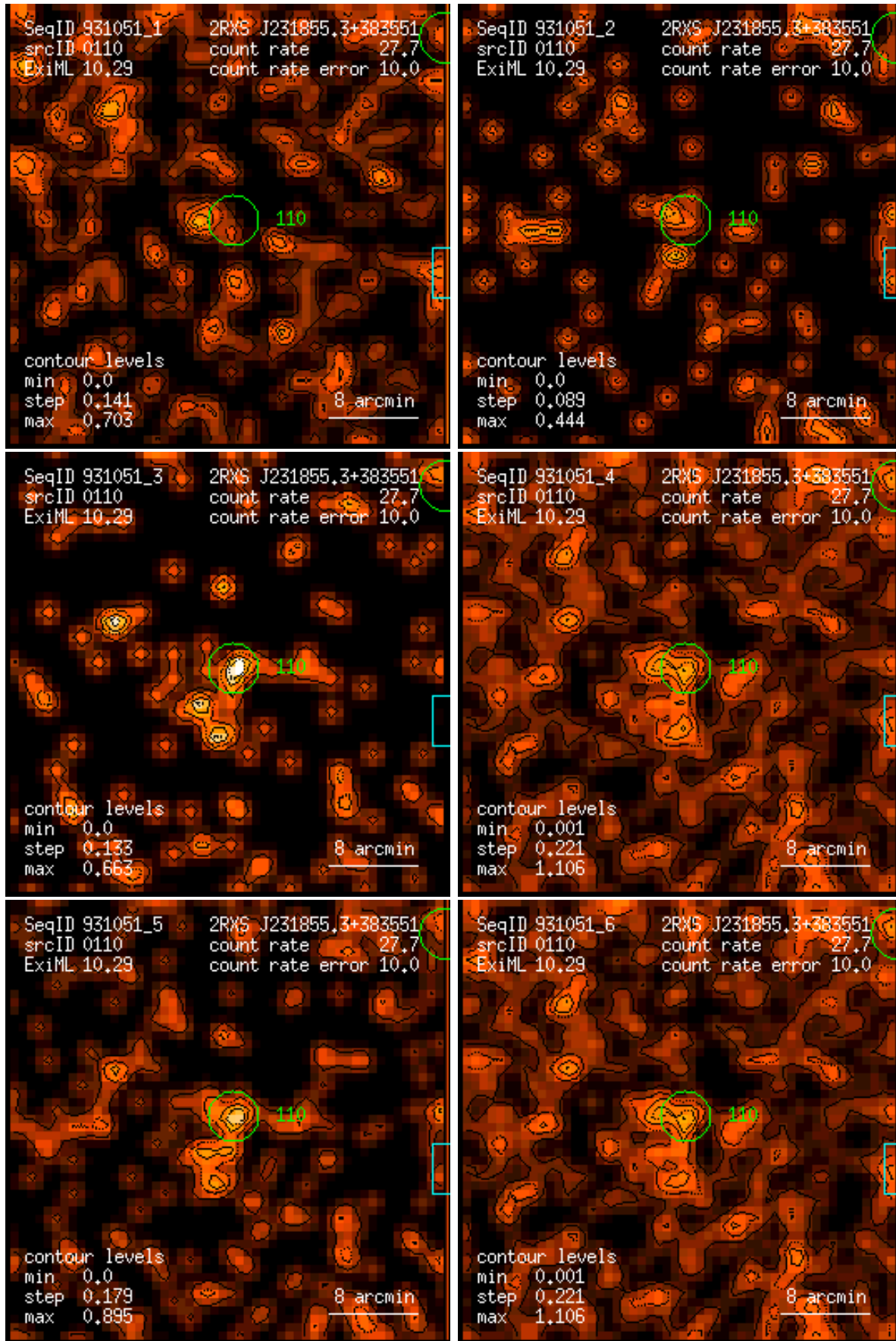
Figure 110: RASS 931051: detection 0110: band rate images, Gaussian filter: (1) PSPC channels 11 – 41, (2) 52 – 90, (3) 91 – 201, (4) 11 – 235, (5) 52 – 201, (6) 11 – 201. Broad band rates in counts/ks. Band rate contour levels in counts/ks/arcmin 2 .
