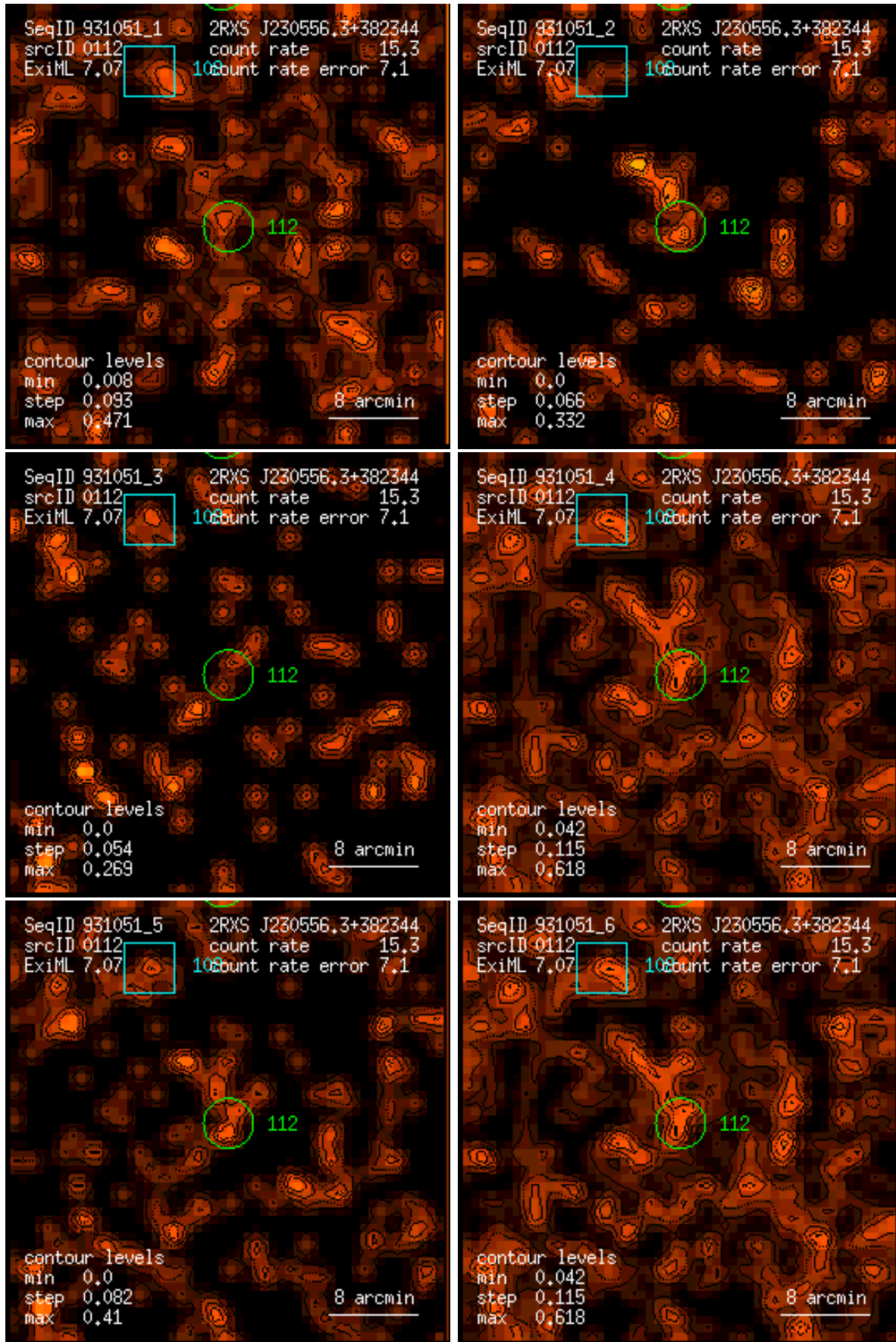
Figure 112: RASS 931051: detection 0112: band rate images, Gaussian filter: (1) PSPC channels 11 – 41, (2) 52 – 90, (3) 91 – 201, (4) 11 – 235, (5) 52 – 201, (6) 11 – 201. Broad band rates in counts/ks. Band rate contour levels in counts/ks/arcmin 2 .
