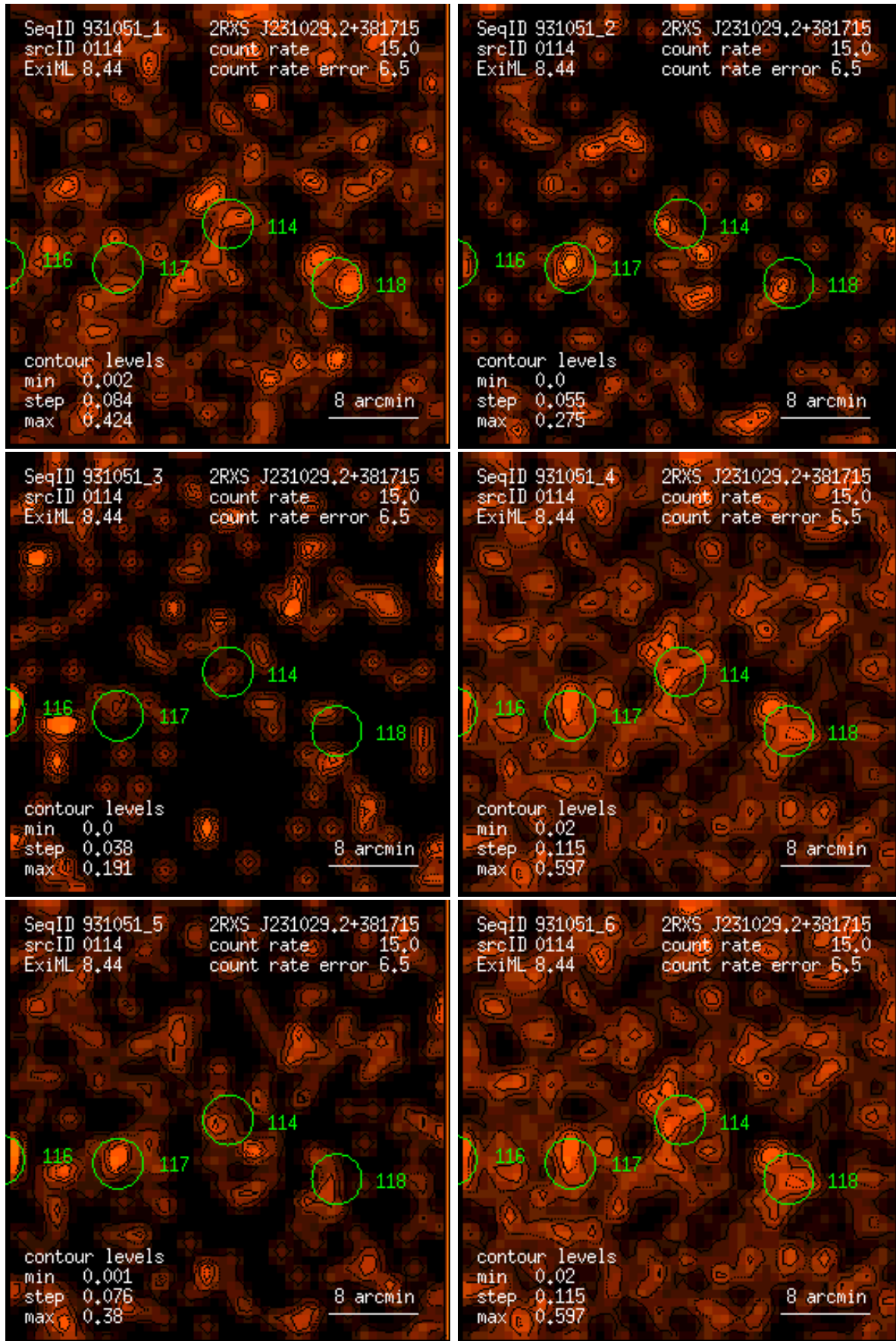
Figure 114: RASS 931051: detection 0114: band rate images, Gaussian filter: (1) PSPC channels 11 – 41, (2) 52 – 90, (3) 91 – 201, (4) 11 – 235, (5) 52 – 201, (6) 11 – 201. Broad band rates in counts/ks. Band rate contour levels in counts/ks/arcmin 2 .
