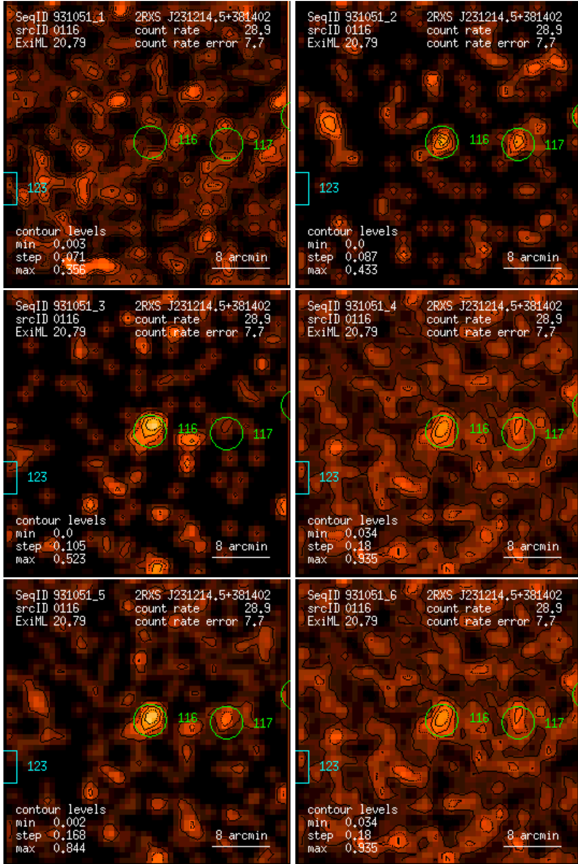
Figure 116: RASS 931051: detection 0116: band rate images, Gaussian filter: (1) PSPC channels 11 – 41, (2) 52 – 90, (3) 91 – 201, (4) 11 – 235, (5) 52 – 201, (6) 11 – 201. Broad band rates in counts/ks. Band rate contour levels in counts/ks/arcmin 2 .
