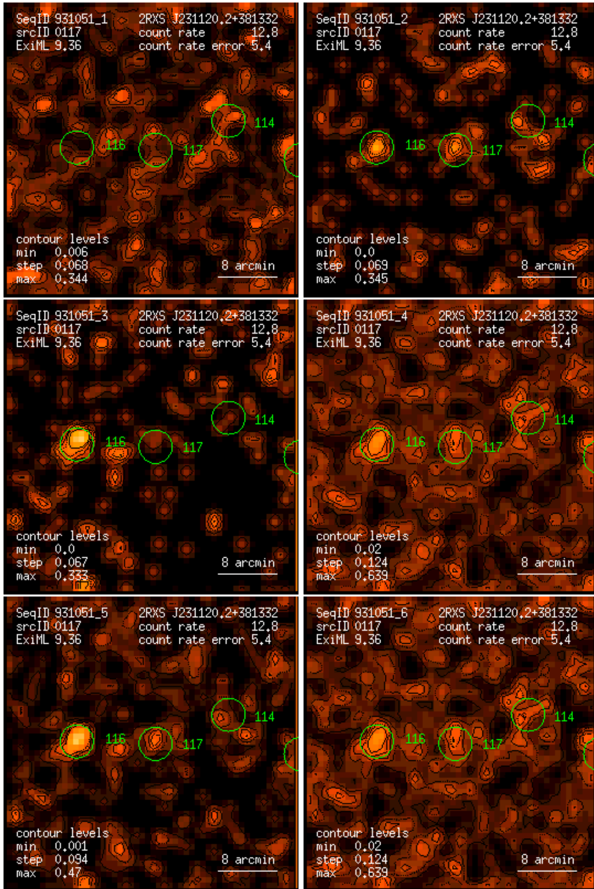
Figure 117: RASS 931051: detection 0117: band rate images, Gaussian filter: (1) PSPC channels 11 – 41, (2) 52 – 90, (3) 91 – 201, (4) 11 – 235, (5) 52 – 201, (6) 11 – 201. Broad band rates in counts/ks. Band rate contour levels in counts/ks/arcmin 2 .
