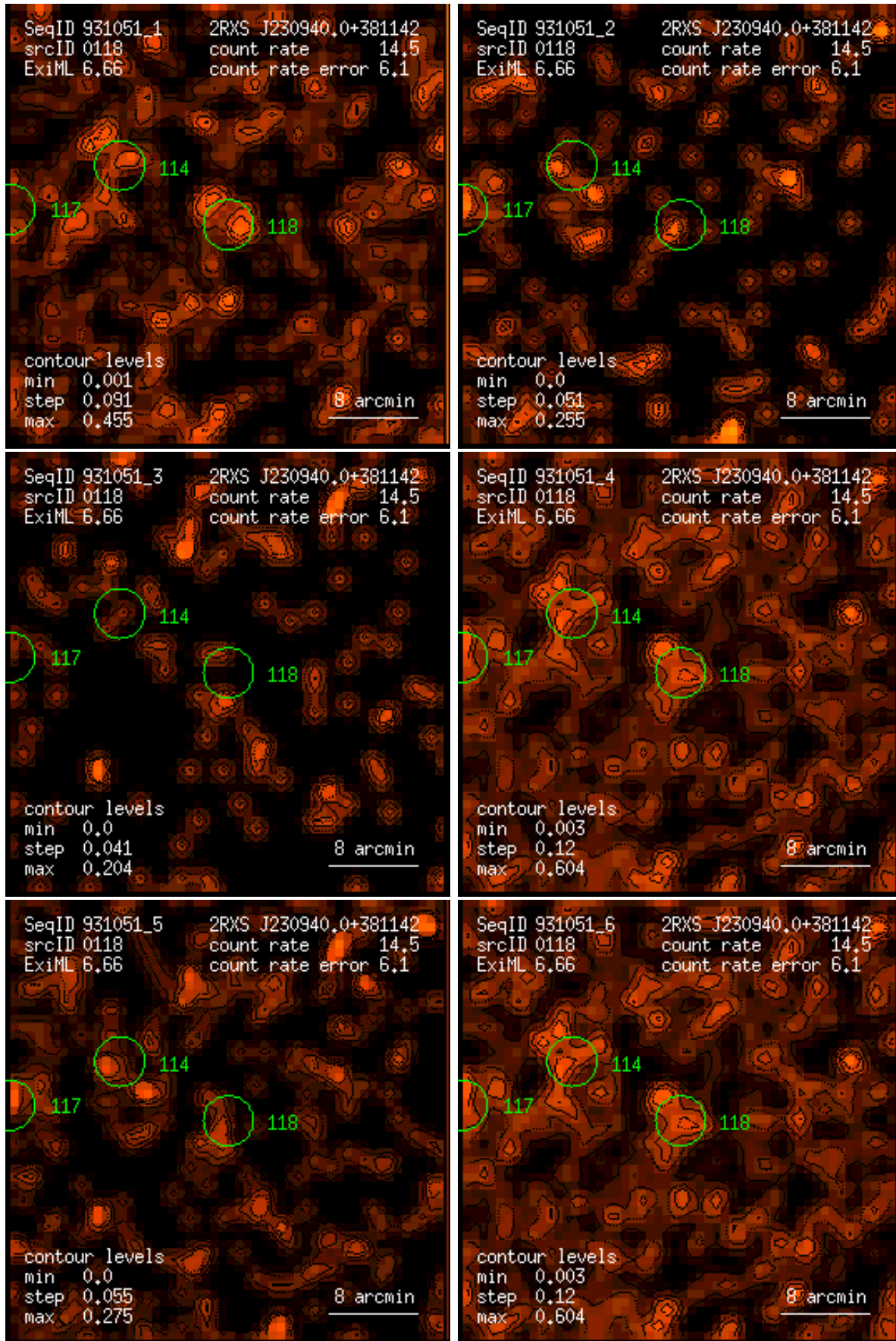
Figure 118: RASS 931051: detection 0118: band rate images, Gaussian filter: (1) PSPC channels 11 – 41, (2) 52 – 90, (3) 91 – 201, (4) 11 – 235, (5) 52 – 201, (6) 11 – 201. Broad band rates in counts/ks. Band rate contour levels in counts/ks/arcmin 2 .
