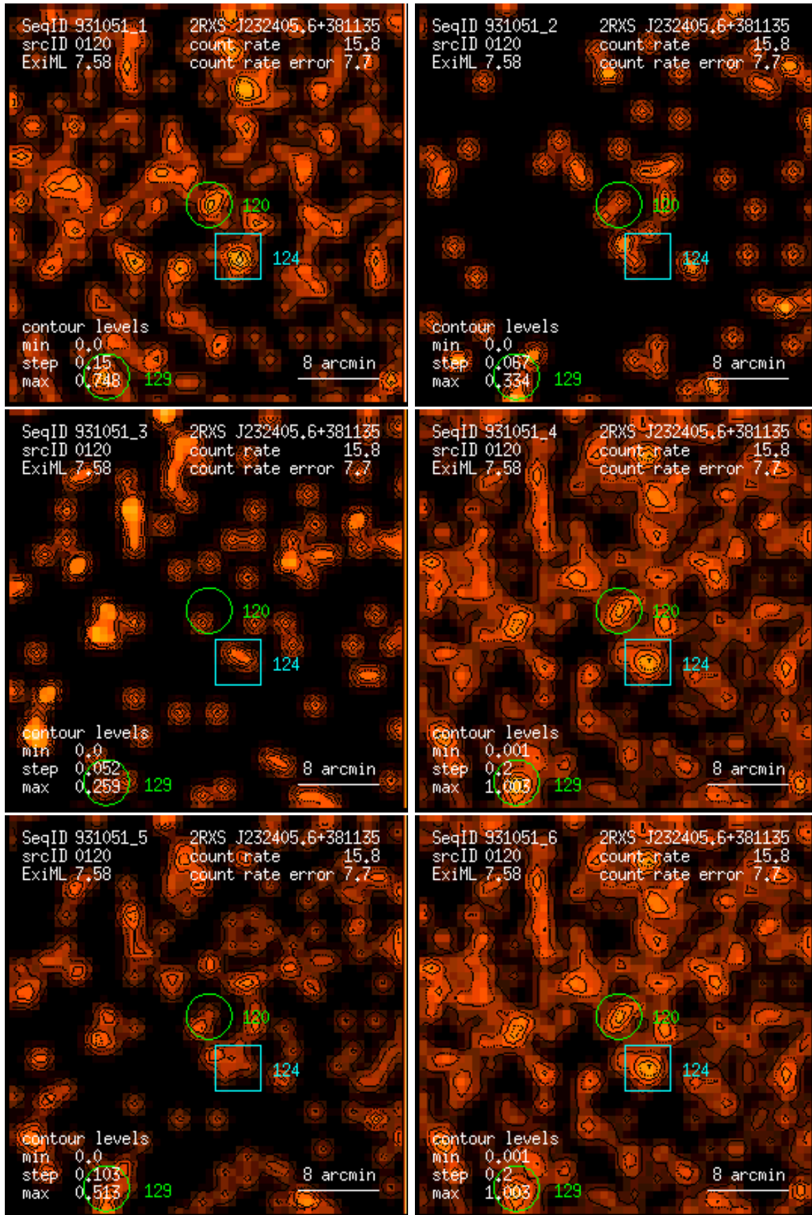
Figure 120: RASS 931051: detection 0120: band rate images, Gaussian filter: (1) PSPC channels 11 – 41, (2) 52 – 90, (3) 91 – 201, (4) 11 – 235, (5) 52 – 201, (6) 11 – 201. Broad band rates in counts/ks. Band rate contour levels in counts/ks/arcmin 2 .
