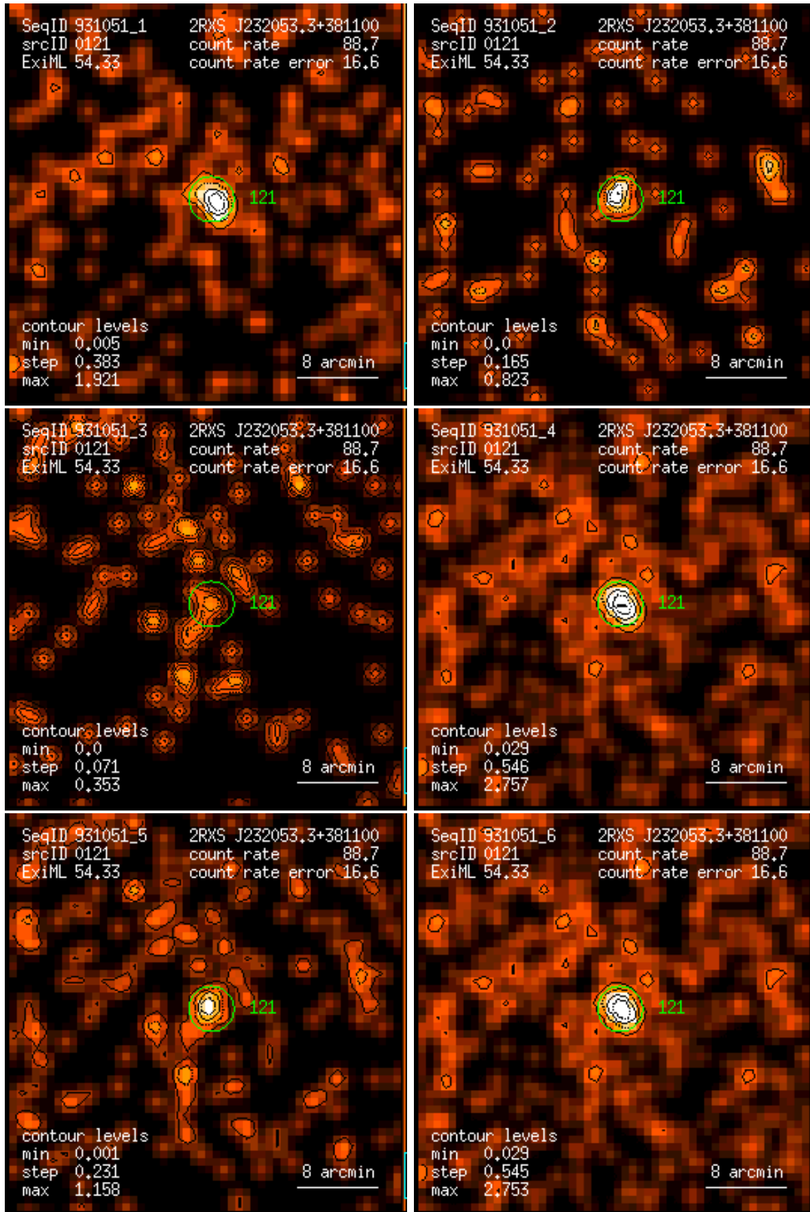
Figure 121: RASS 931051: detection 0121: band rate images, Gaussian filter: (1) PSPC channels 11 – 41, (2) 52 – 90, (3) 91 – 201, (4) 11 – 235, (5) 52 – 201, (6) 11 – 201. Broad band rates in counts/ks. Band rate contour levels in counts/ks/arcmin 2 .
