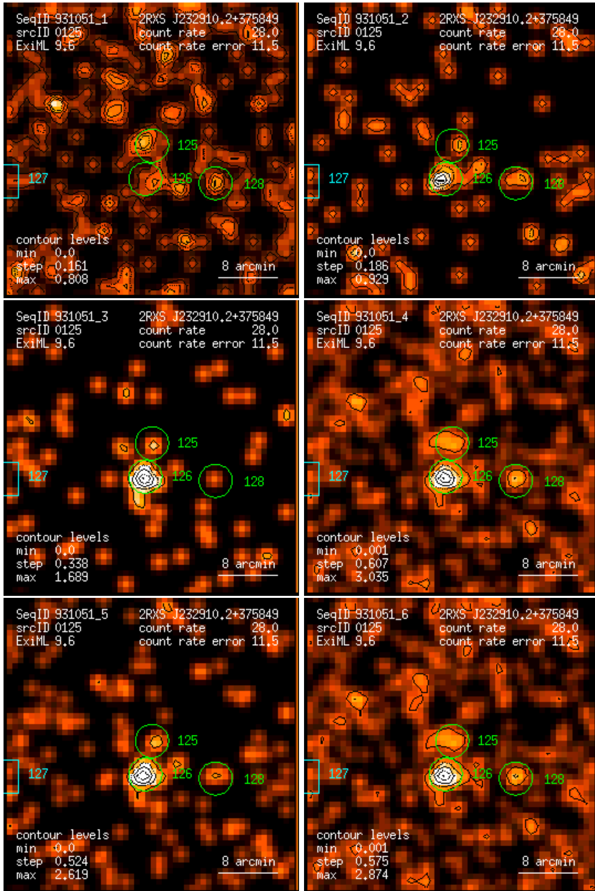
Figure 125: RASS 931051: detection 0125: band rate images, Gaussian filter: (1) PSPC channels 11 – 41, (2) 52 – 90, (3) 91 – 201, (4) 11 – 235, (5) 52 – 201, (6) 11 – 201. Broad band rates in counts/ks. Band rate contour levels in counts/ks/arcmin 2 .
