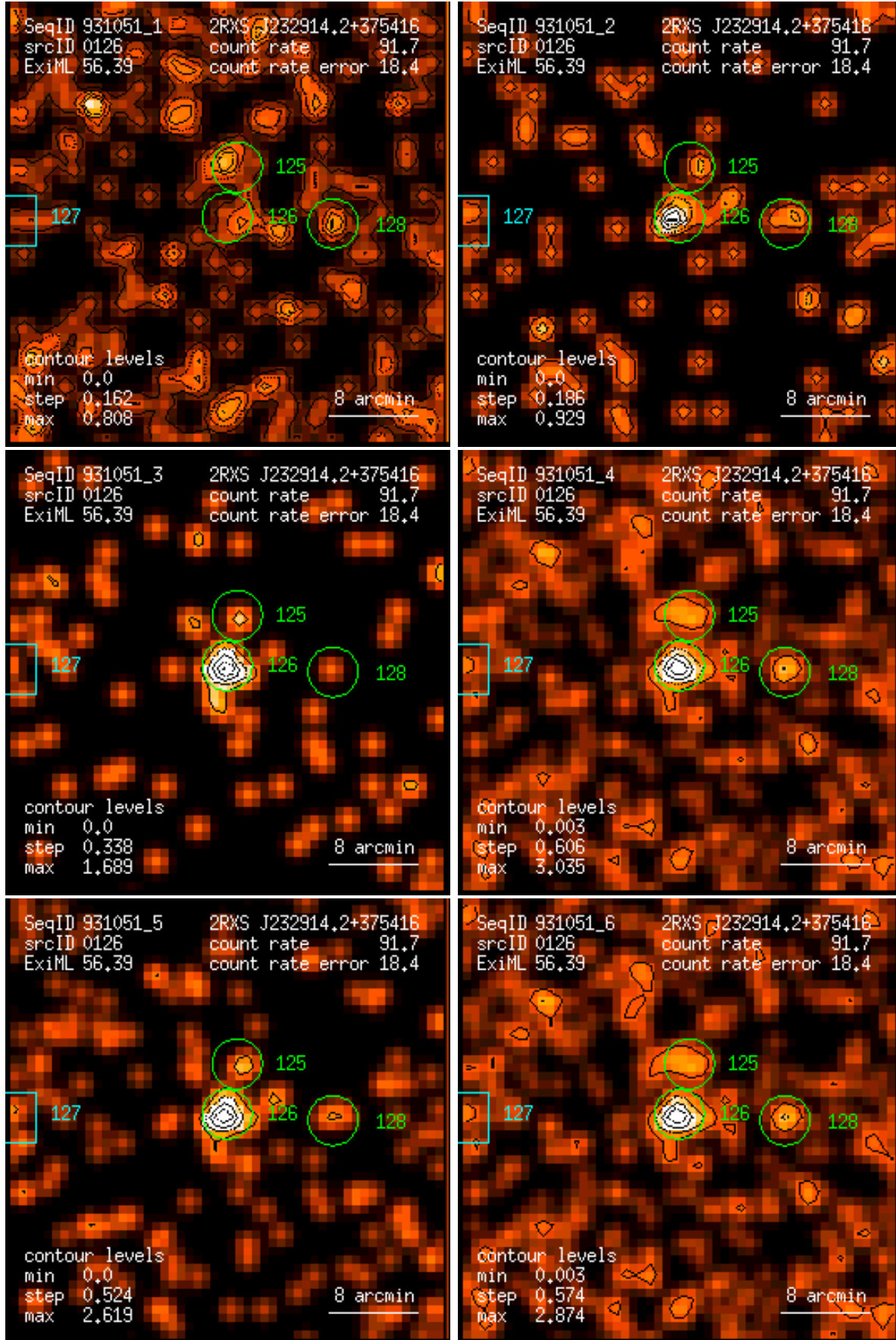
Figure 126: RASS 931051: detection 0126: band rate images, Gaussian filter: (1) PSPC channels 11 – 41, (2) 52 – 90, (3) 91 – 201, (4) 11 – 235, (5) 52 – 201, (6) 11 – 201. Broad band rates in counts/ks. Band rate contour levels in counts/ks/arcmin 2 .
