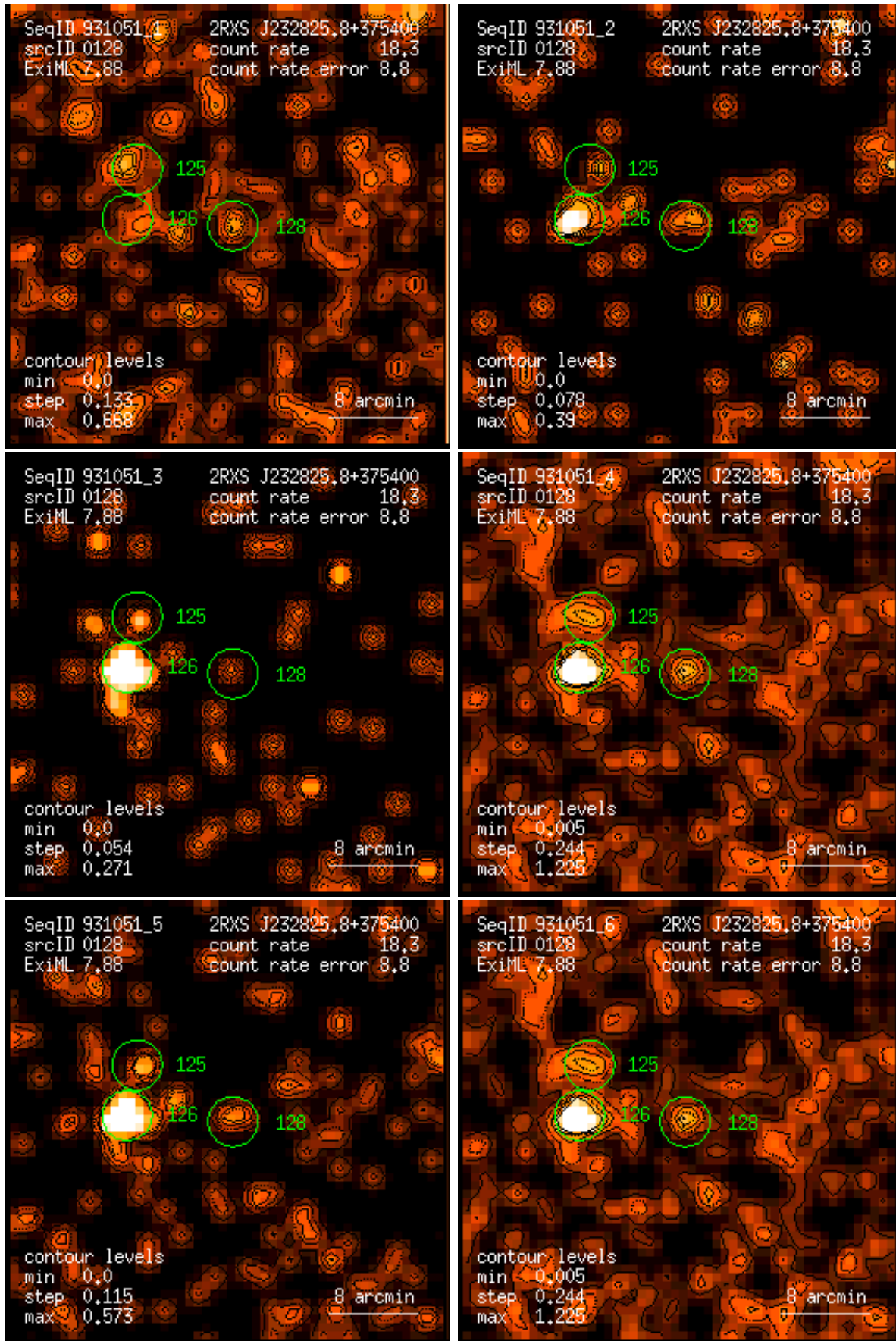
Figure 128: RASS 931051: detection 0128: band rate images, Gaussian filter: (1) PSPC channels 11 – 41, (2) 52 – 90, (3) 91 – 201, (4) 11 – 235, (5) 52 – 201, (6) 11 – 201. Broad band rates in counts/ks. Band rate contour levels in counts/ks/arcmin 2 .
