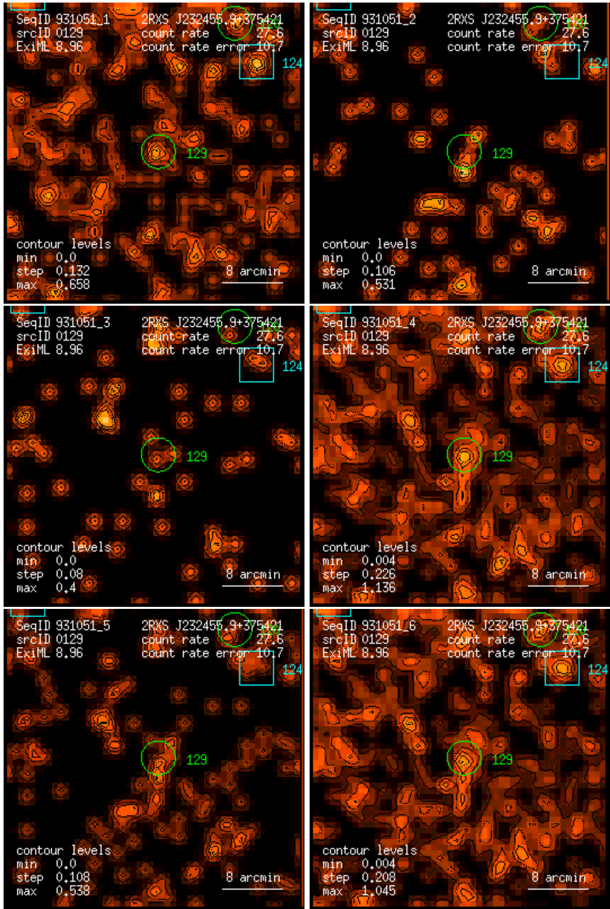
Figure 129: RASS 931051: detection 0129: band rate images, Gaussian filter: (1) PSPC channels 11 – 41, (2) 52 – 90, (3) 91 – 201, (4) 11 – 235, (5) 52 – 201, (6) 11 – 201. Broad band rates in counts/ks. Band rate contour levels in counts/ks/arcmin 2 .
