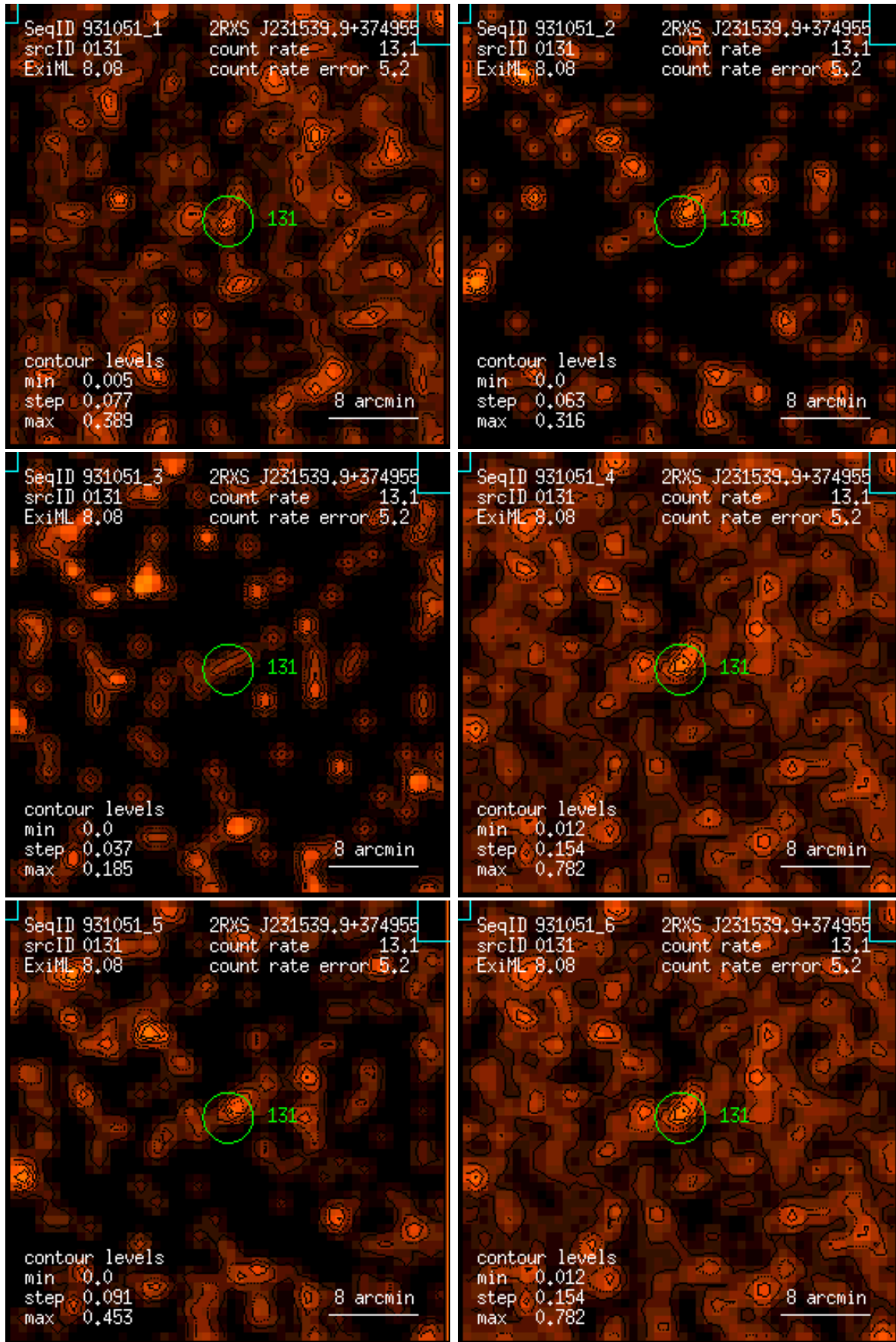
Figure 131: RASS 931051: detection 0131: band rate images, Gaussian filter: (1) PSPC channels 11 – 41, (2) 52 – 90, (3) 91 – 201, (4) 11 – 235, (5) 52 – 201, (6) 11 – 201. Broad band rates in counts/ks. Band rate contour levels in counts/ks/arcmin 2 .
