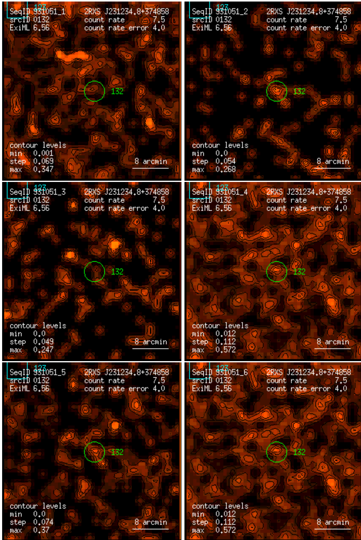
Figure 132: RASS 931051: detection 0132: band rate images, Gaussian filter: (1) PSPC channels 11 – 41, (2) 52 – 90, (3) 91 – 201, (4) 11 – 235, (5) 52 – 201, (6) 11 – 201. Broad band rates in counts/ks. Band rate contour levels in counts/ks/arcmin 2 .
