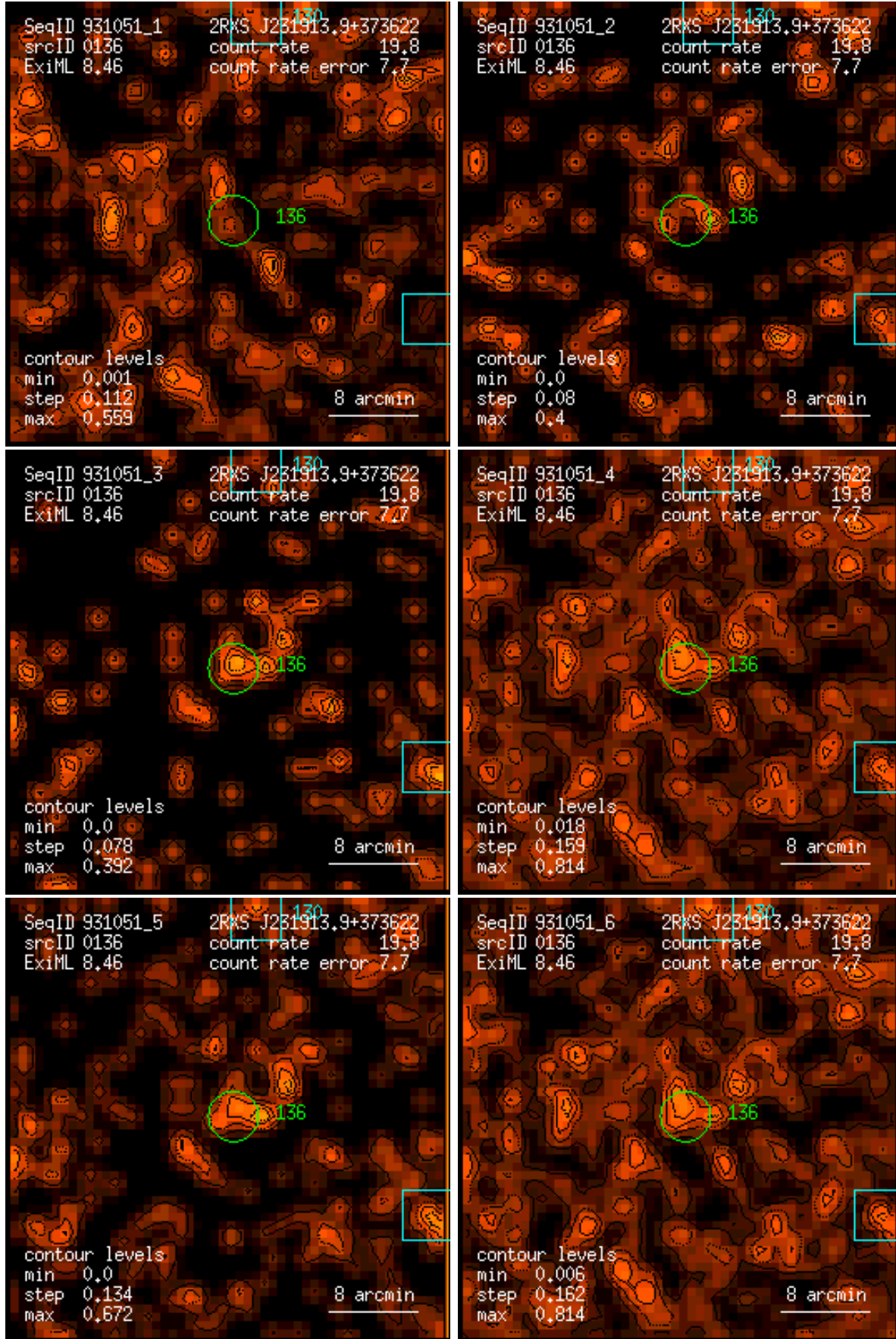
Figure 136: RASS 931051: detection 0136: band rate images, Gaussian filter: (1) PSPC channels 11 – 41, (2) 52 – 90, (3) 91 – 201, (4) 11 – 235, (5) 52 – 201, (6) 11 – 201. Broad band rates in counts/ks. Band rate contour levels in counts/ks/arcmin 2 .
