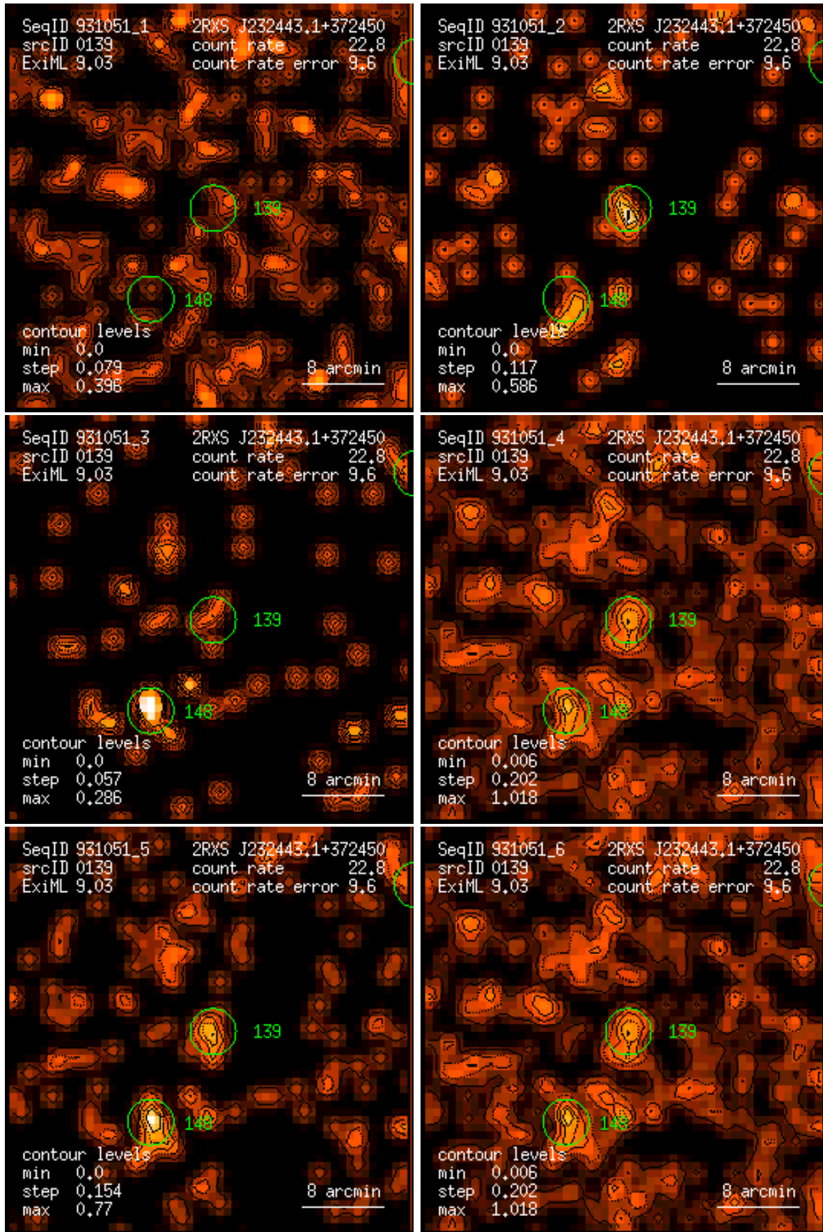
Figure 139: RASS 931051: detection 0139: band rate images, Gaussian filter: (1) PSPC channels 11 – 41, (2) 52 – 90, (3) 91 – 201, (4) 11 – 235, (5) 52 – 201, (6) 11 – 201. Broad band rates in counts/ks. Band rate contour levels in counts/ks/arcmin 2 .
