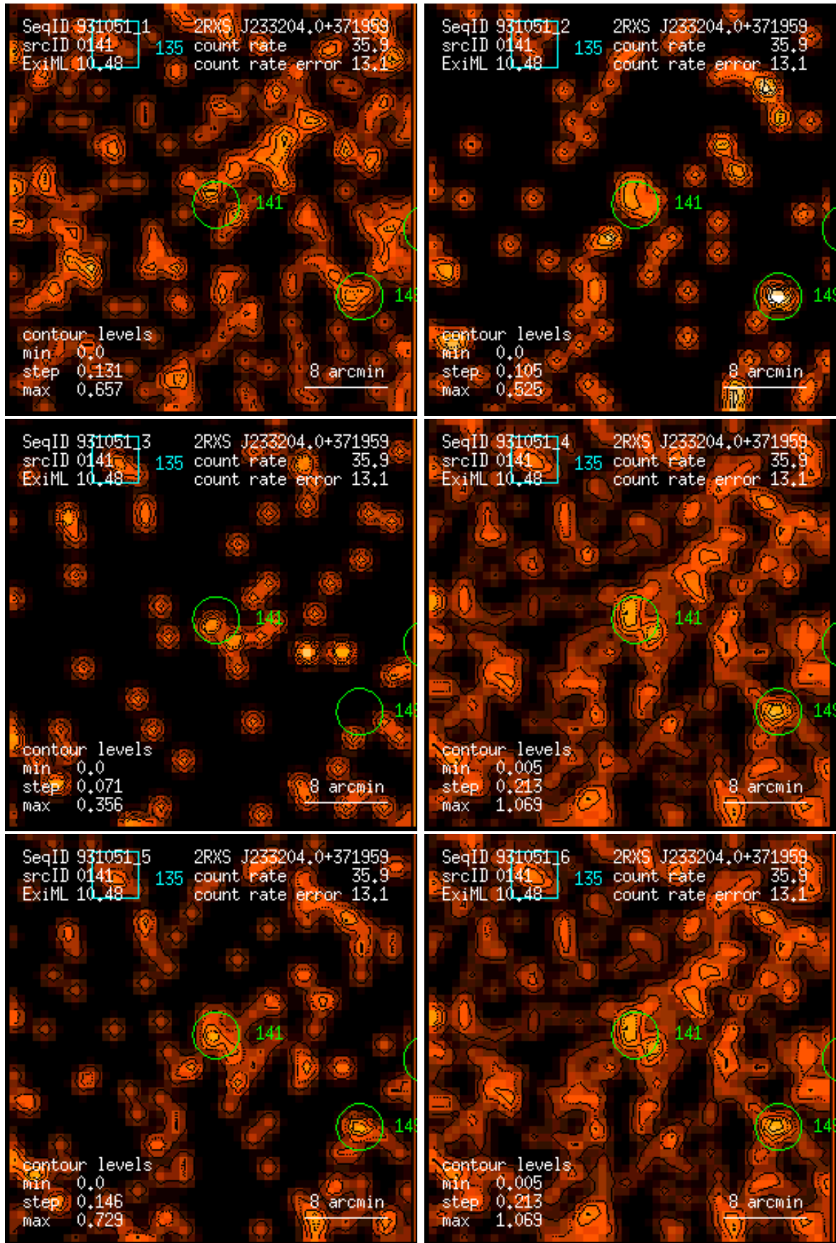
Figure 141: RASS 931051: detection 0141: band rate images, Gaussian filter: (1) PSPC channels 11 – 41, (2) 52 – 90, (3) 91 – 201, (4) 11 – 235, (5) 52 – 201, (6) 11 – 201. Broad band rates in counts/ks. Band rate contour levels in counts/ks/arcmin 2 .
