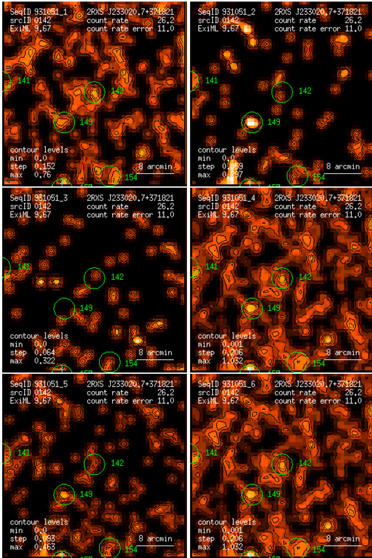
Figure 142: RASS 931051: detection 0142: band rate images, Gaussian filter: (1) PSPC channels 11 – 41, (2) 52 – 90, (3) 91 – 201, (4) 11 – 235, (5) 52 – 201, (6) 11 – 201. Broad band rates in counts/ks. Band rate contour levels in counts/ks/arcmin 2 .
