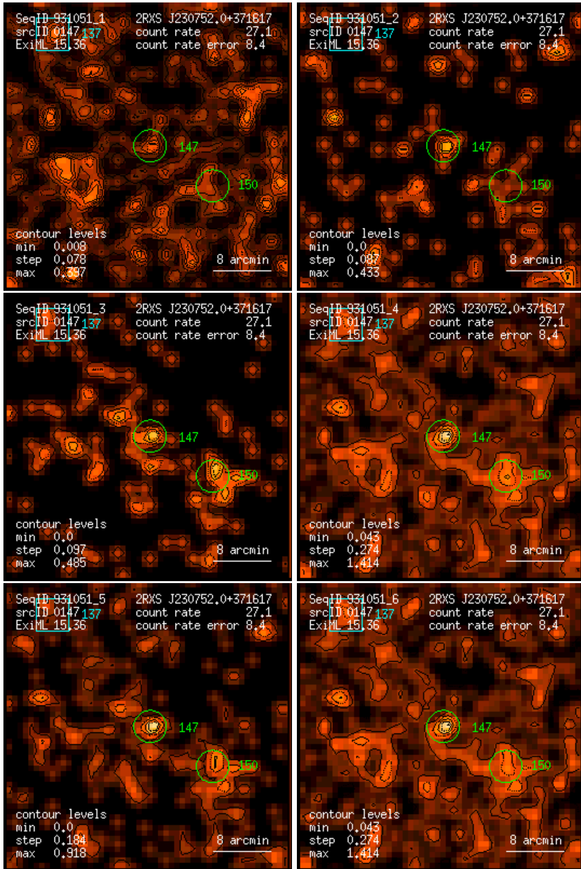
Figure 147: RASS 931051: detection 0147: band rate images, Gaussian filter: (1) PSPC channels 11 – 41, (2) 52 – 90, (3) 91 – 201, (4) 11 – 235, (5) 52 – 201, (6) 11 – 201. Broad band rates in counts/ks. Band rate contour levels in counts/ks/arcmin 2 .
