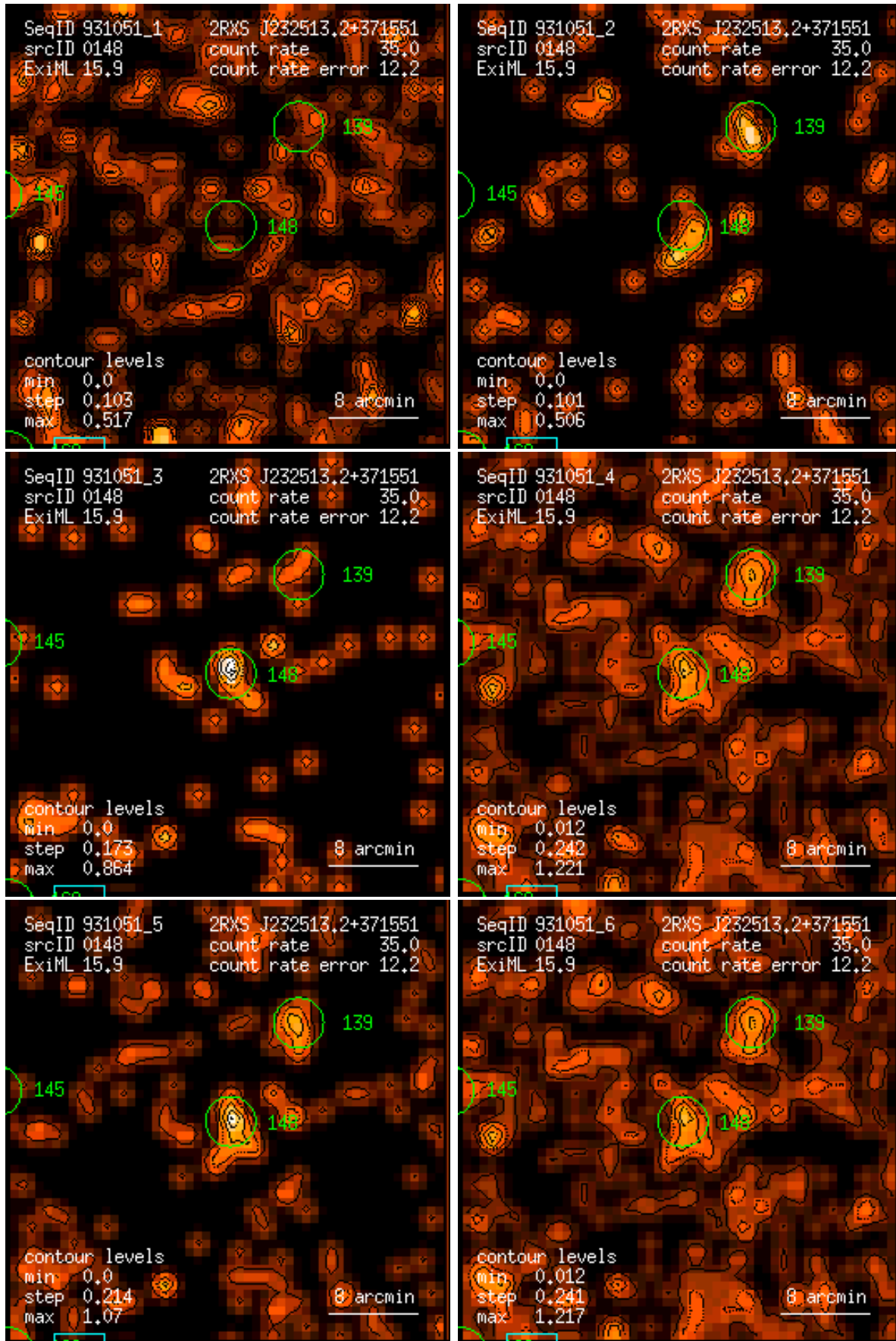
Figure 148: RASS 931051: detection 0148: band rate images, Gaussian filter: (1) PSPC channels 11 – 41, (2) 52 – 90, (3) 91 – 201, (4) 11 – 235, (5) 52 – 201, (6) 11 – 201. Broad band rates in counts/ks. Band rate contour levels in counts/ks/arcmin 2 .
