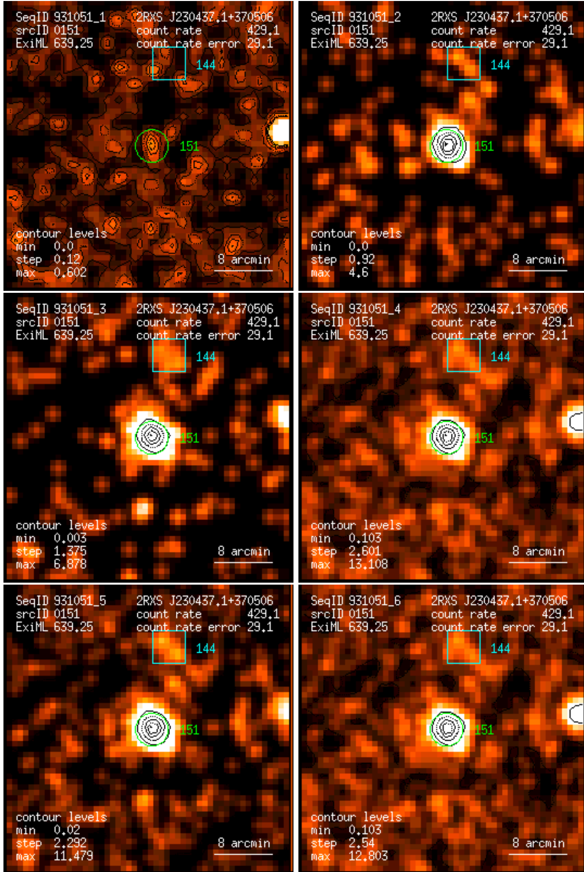
Figure 151: RASS 931051: detection 0151: band rate images, Gaussian filter: (1) PSPC channels 11 – 41, (2) 52 – 90, (3) 91 – 201, (4) 11 – 235, (5) 52 – 201, (6) 11 – 201. Broad band rates in counts/ks. Band rate contour levels in counts/ks/arcmin 2 .
