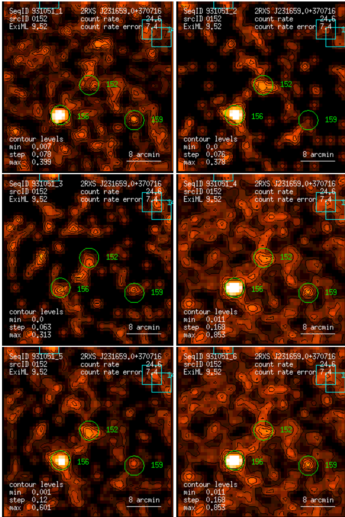
Figure 152: RASS 931051: detection 0152: band rate images, Gaussian filter: (1) PSPC channels 11 – 41, (2) 52 – 90, (3) 91 – 201, (4) 11 – 235, (5) 52 – 201, (6) 11 – 201. Broad band rates in counts/ks. Band rate contour levels in counts/ks/arcmin 2 .
