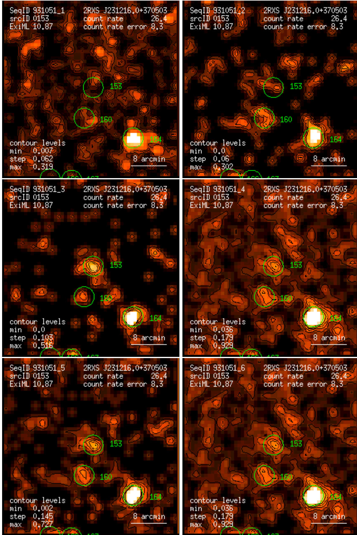
Figure 153: RASS 931051: detection 0153: band rate images, Gaussian filter: (1) PSPC channels 11 – 41, (2) 52 – 90, (3) 91 – 201, (4) 11 – 235, (5) 52 – 201, (6) 11 – 201. Broad band rates in counts/ks. Band rate contour levels in counts/ks/arcmin 2 .
