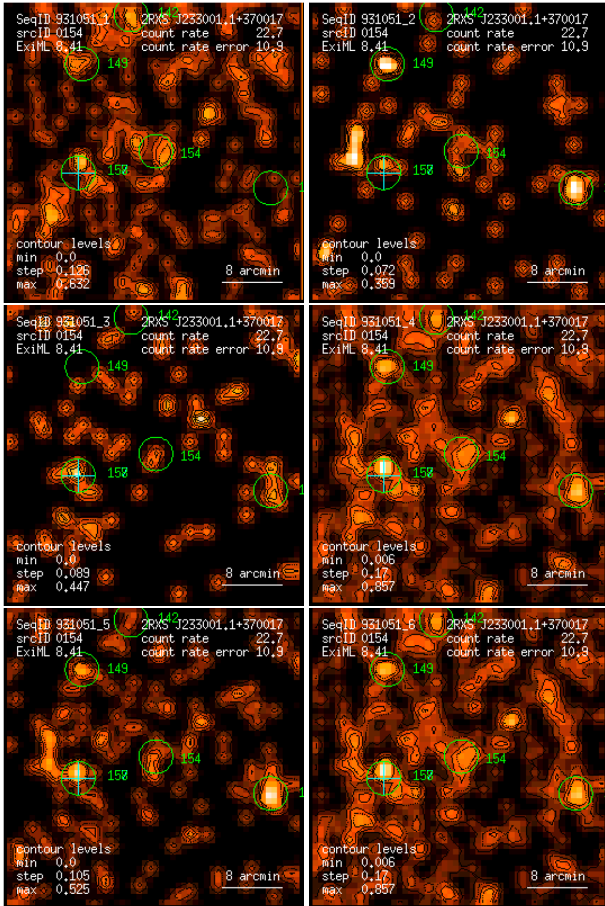
Figure 154: RASS 931051: detection 0154: band rate images, Gaussian filter: (1) PSPC channels 11 – 41, (2) 52 – 90, (3) 91 – 201, (4) 11 – 235, (5) 52 – 201, (6) 11 – 201. Broad band rates in counts/ks. Band rate contour levels in counts/ks/arcmin 2 .
