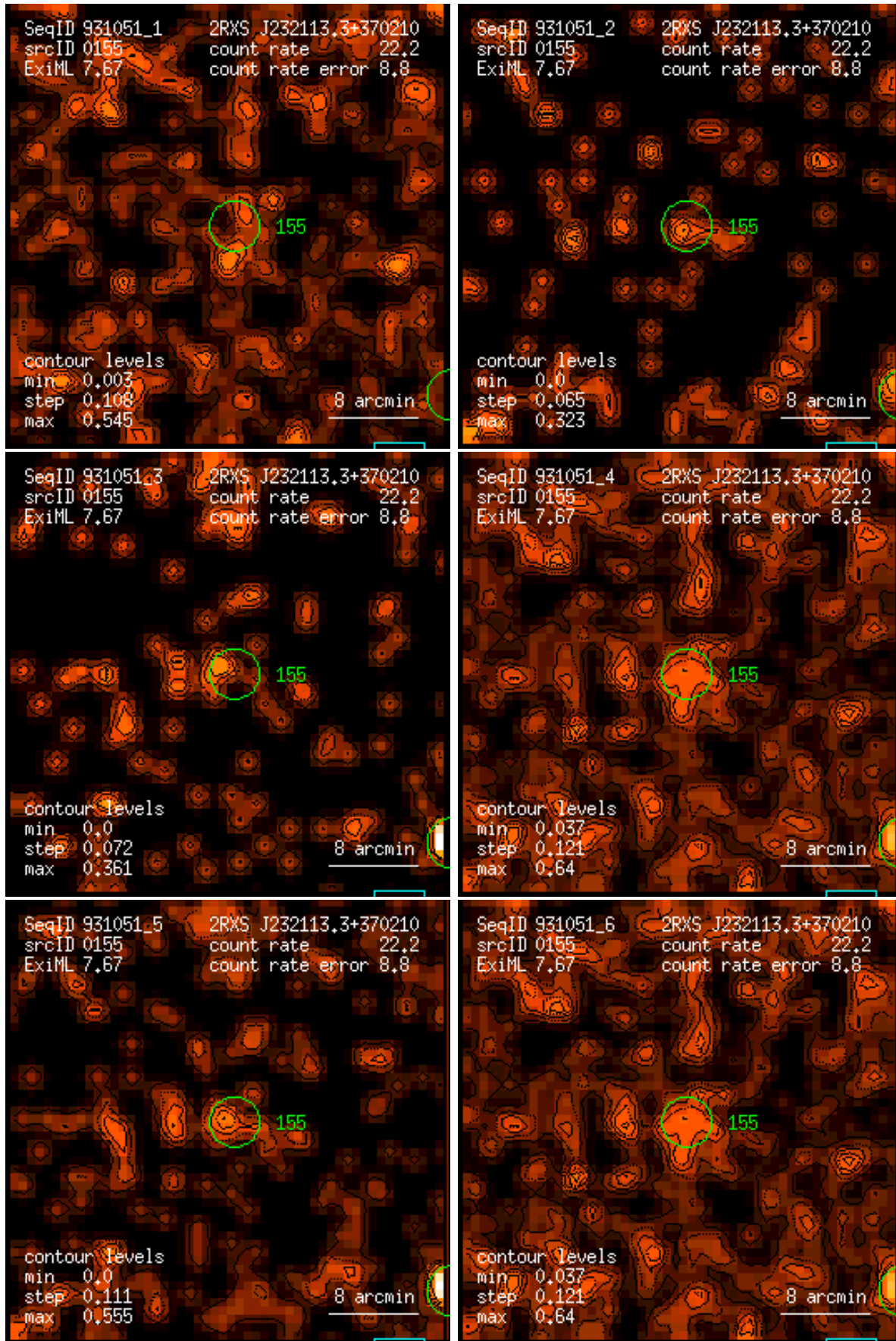
Figure 155: RASS 931051: detection 0155: band rate images, Gaussian filter: (1) PSPC channels 11 – 41, (2) 52 – 90, (3) 91 – 201, (4) 11 – 235, (5) 52 – 201, (6) 11 – 201. Broad band rates in counts/ks. Band rate contour levels in counts/ks/arcmin 2 .
