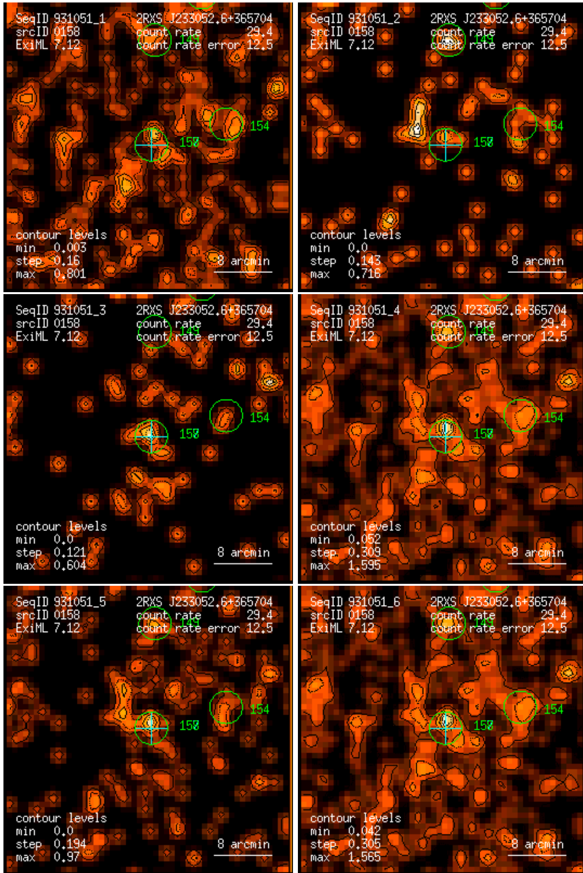
Figure 158: RASS 931051: detection 0158: band rate images, Gaussian filter: (1) PSPC channels 11 – 41, (2) 52 – 90, (3) 91 – 201, (4) 11 – 235, (5) 52 – 201, (6) 11 – 201. Broad band rates in counts/ks. Band rate contour levels in counts/ks/arcmin 2 .
