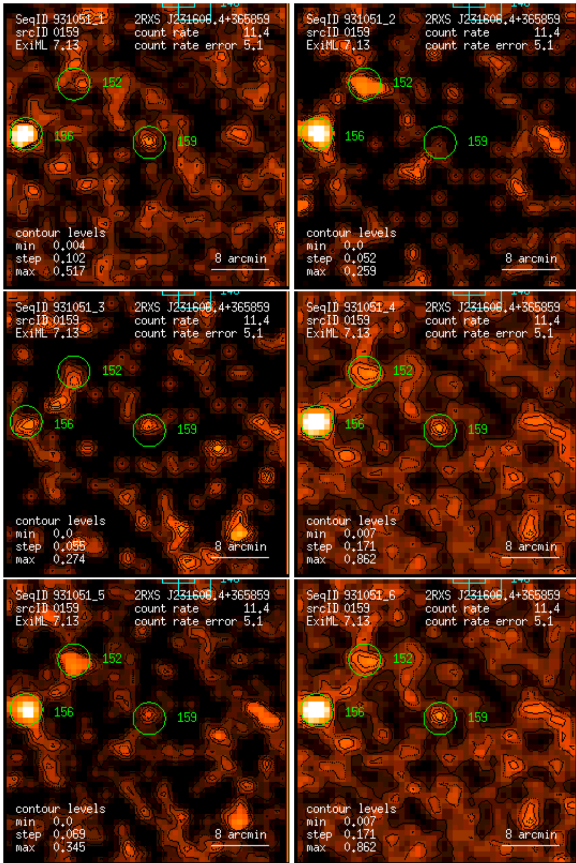
Figure 159: RASS 931051: detection 0159: band rate images, Gaussian filter: (1) PSPC channels 11 – 41, (2) 52 – 90, (3) 91 – 201, (4) 11 – 235, (5) 52 – 201, (6) 11 – 201. Broad band rates in counts/ks. Band rate contour levels in counts/ks/arcmin 2 .
