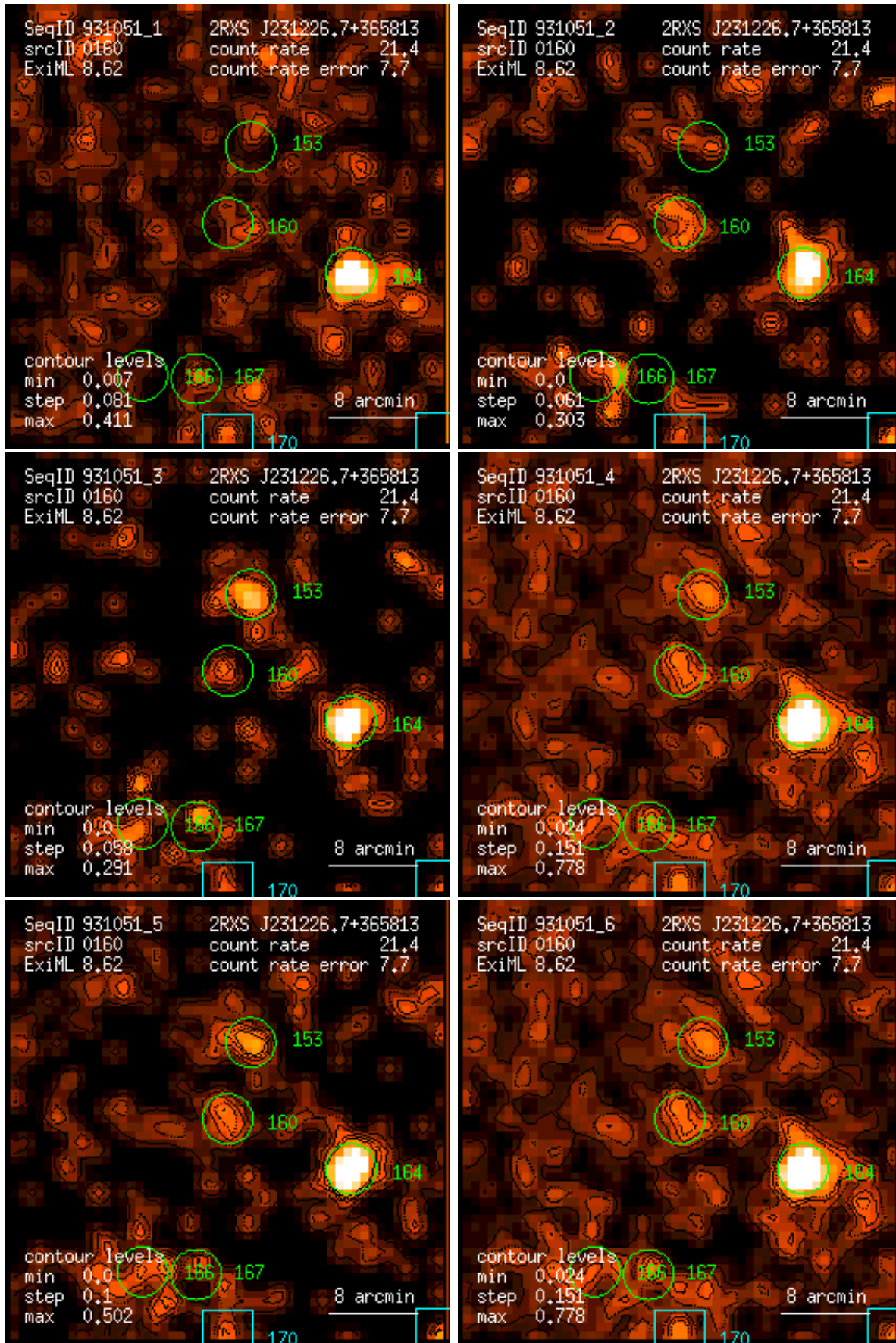
Figure 160: RASS 931051: detection 0160: band rate images, Gaussian filter: (1) PSPC channels 11 – 41, (2) 52 – 90, (3) 91 – 201, (4) 11 – 235, (5) 52 – 201, (6) 11 – 201. Broad band rates in counts/ks. Band rate contour levels in counts/ks/arcmin 2 .
