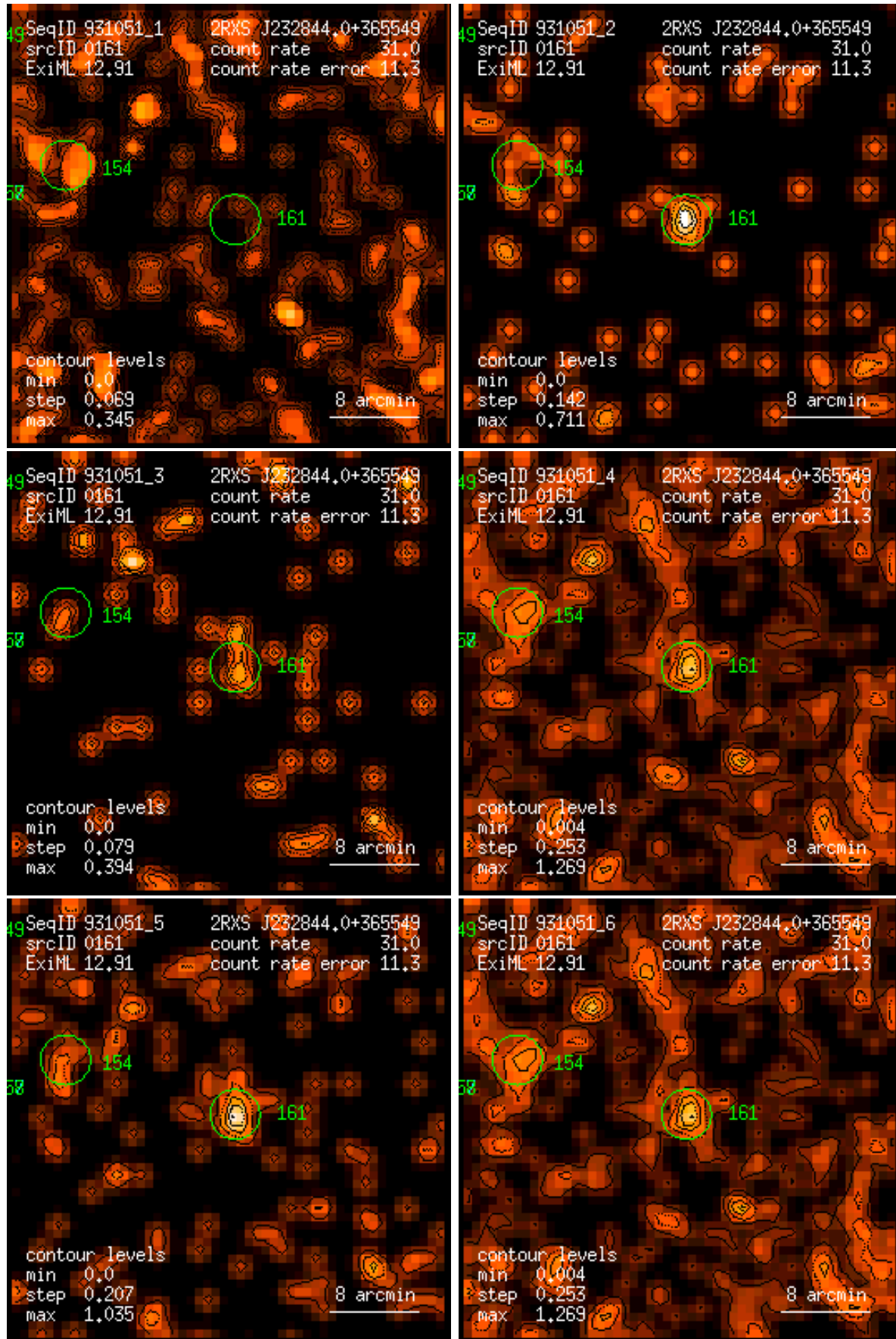
Figure 161: RASS 931051: detection 0161: band rate images, Gaussian filter: (1) PSPC channels 11 – 41, (2) 52 – 90, (3) 91 – 201, (4) 11 – 235, (5) 52 – 201, (6) 11 – 201. Broad band rates in counts/ks. Band rate contour levels in counts/ks/arcmin 2 .
