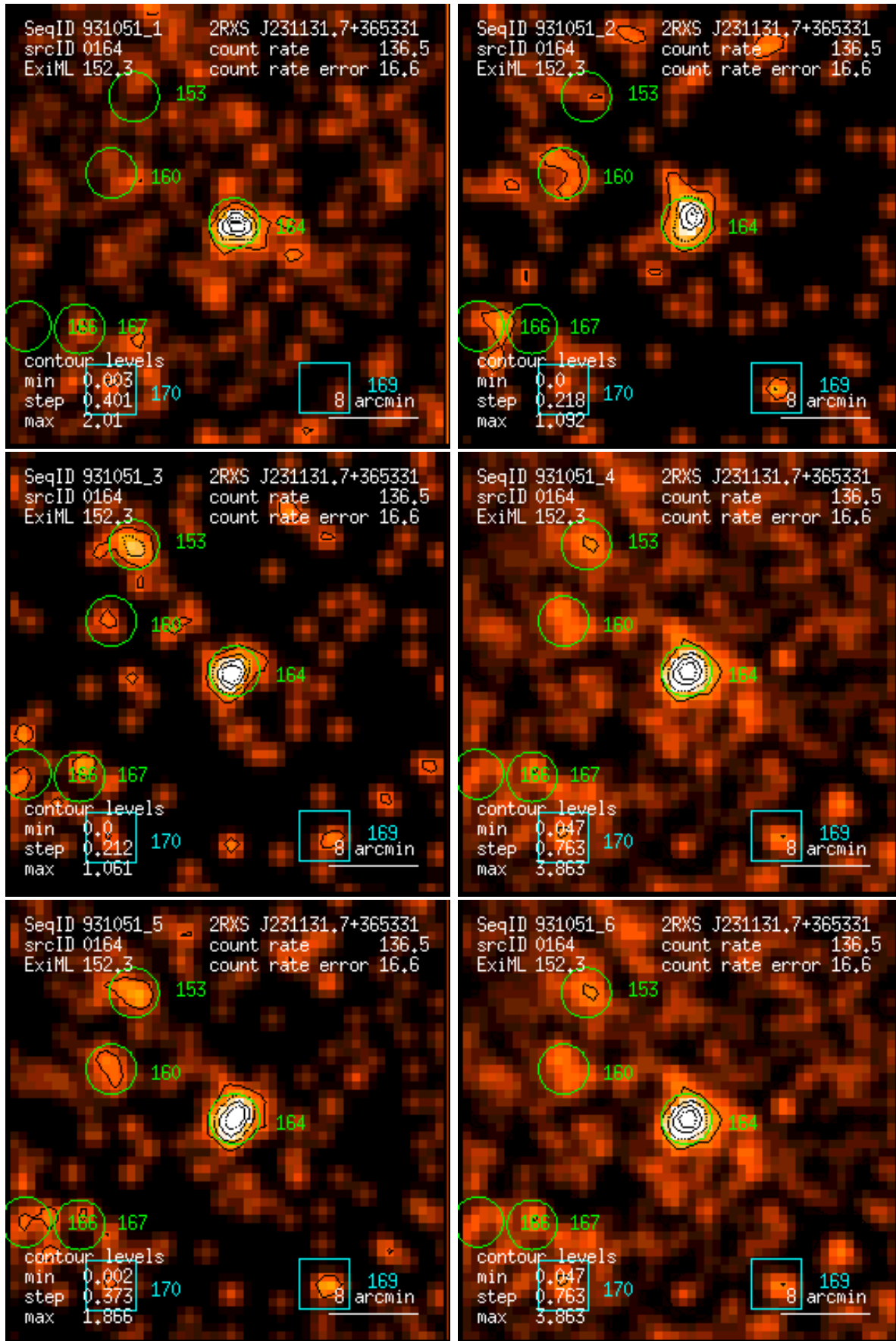
Figure 164: RASS 931051: detection 0164: band rate images, Gaussian filter: (1) PSPC channels 11 – 41, (2) 52 – 90, (3) 91 – 201, (4) 11 – 235, (5) 52 – 201, (6) 11 – 201. Broad band rates in counts/ks. Band rate contour levels in counts/ks/arcmin 2 .
