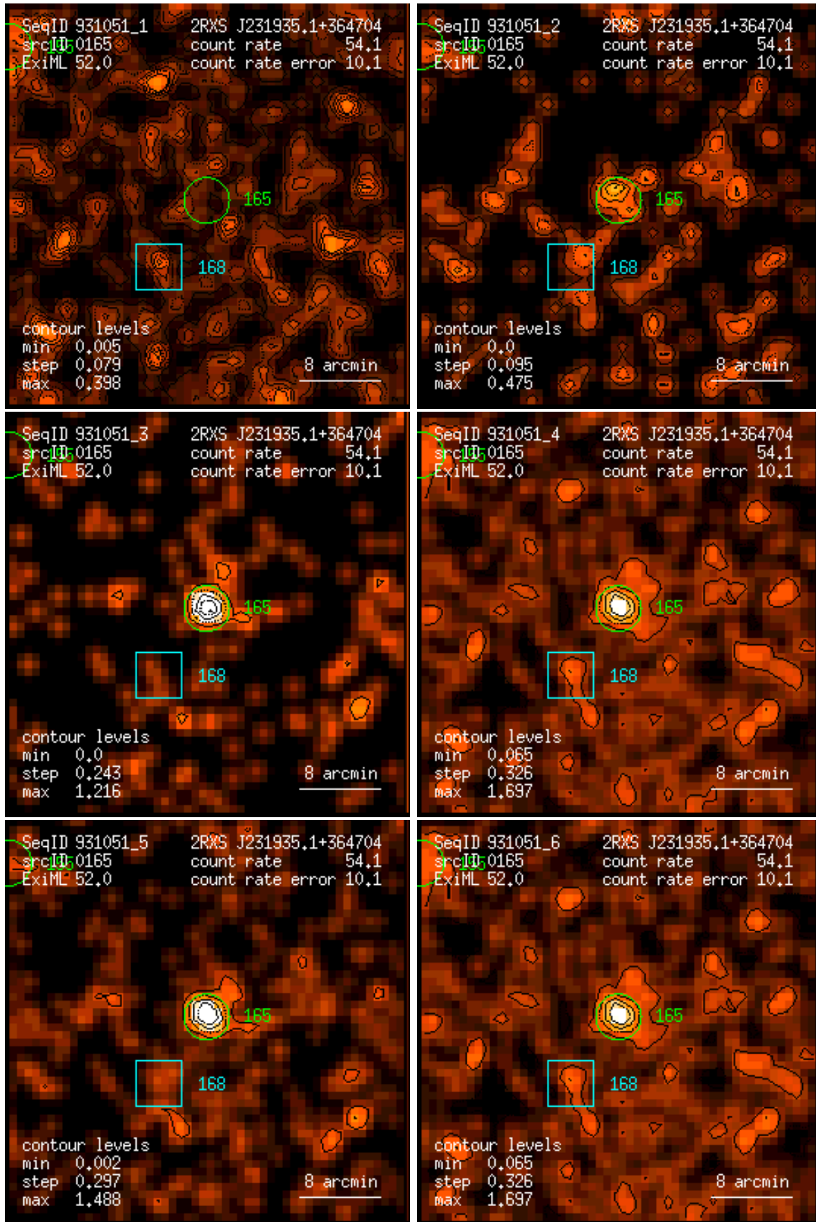
Figure 165: RASS 931051: detection 0165: band rate images, Gaussian filter: (1) PSPC channels 11 – 41, (2) 52 – 90, (3) 91 – 201, (4) 11 – 235, (5) 52 – 201, (6) 11 – 201. Broad band rates in counts/ks. Band rate contour levels in counts/ks/arcmin 2 .
