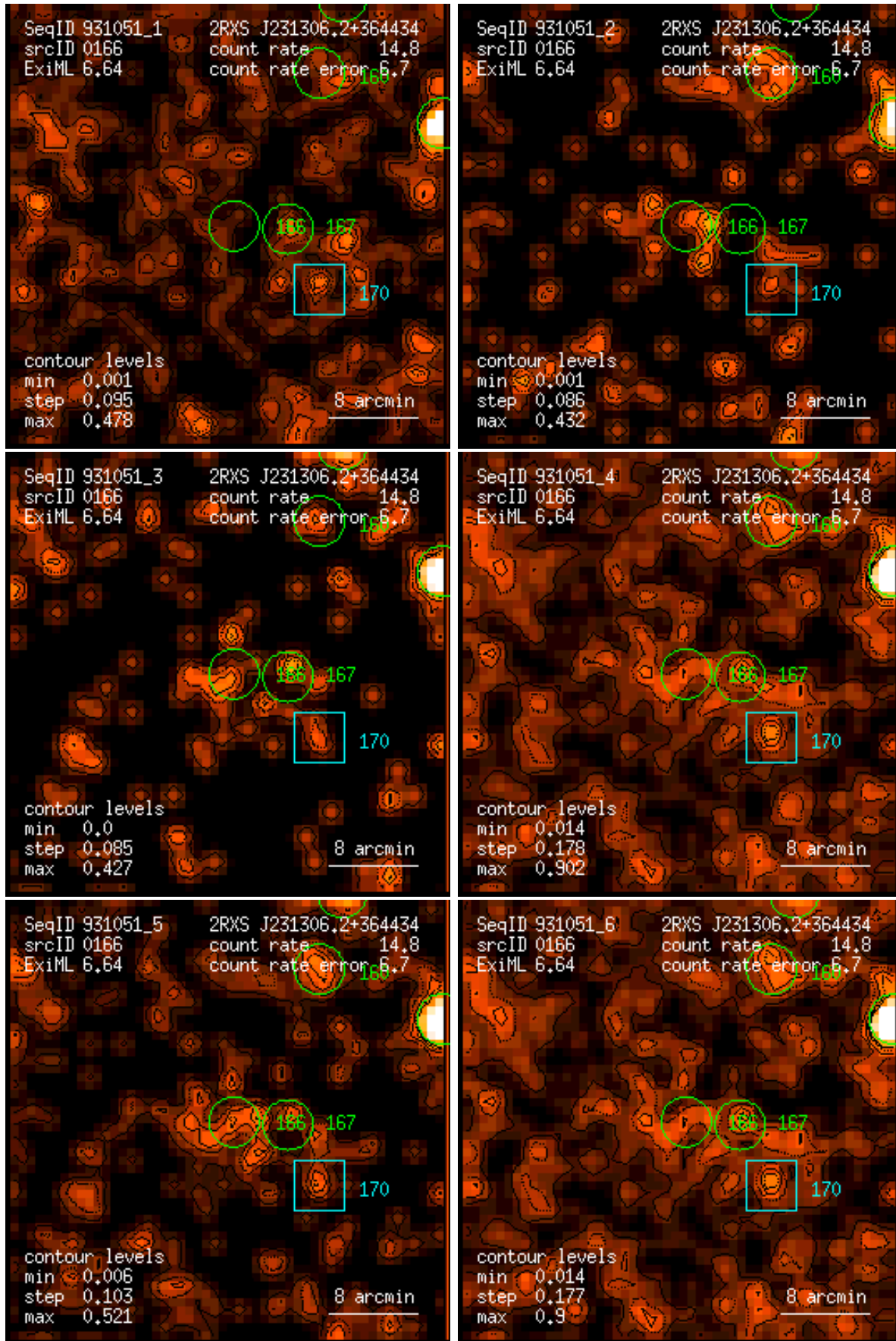
Figure 166: RASS 931051: detection 0166: band rate images, Gaussian filter: (1) PSPC channels 11 – 41, (2) 52 – 90, (3) 91 – 201, (4) 11 – 235, (5) 52 – 201, (6) 11 – 201. Broad band rates in counts/ks. Band rate contour levels in counts/ks/arcmin 2 .
